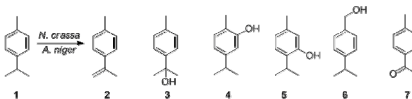
Fig.1. The biotransformation of 1 by N. crassa and A. niger TBUYN-2.
