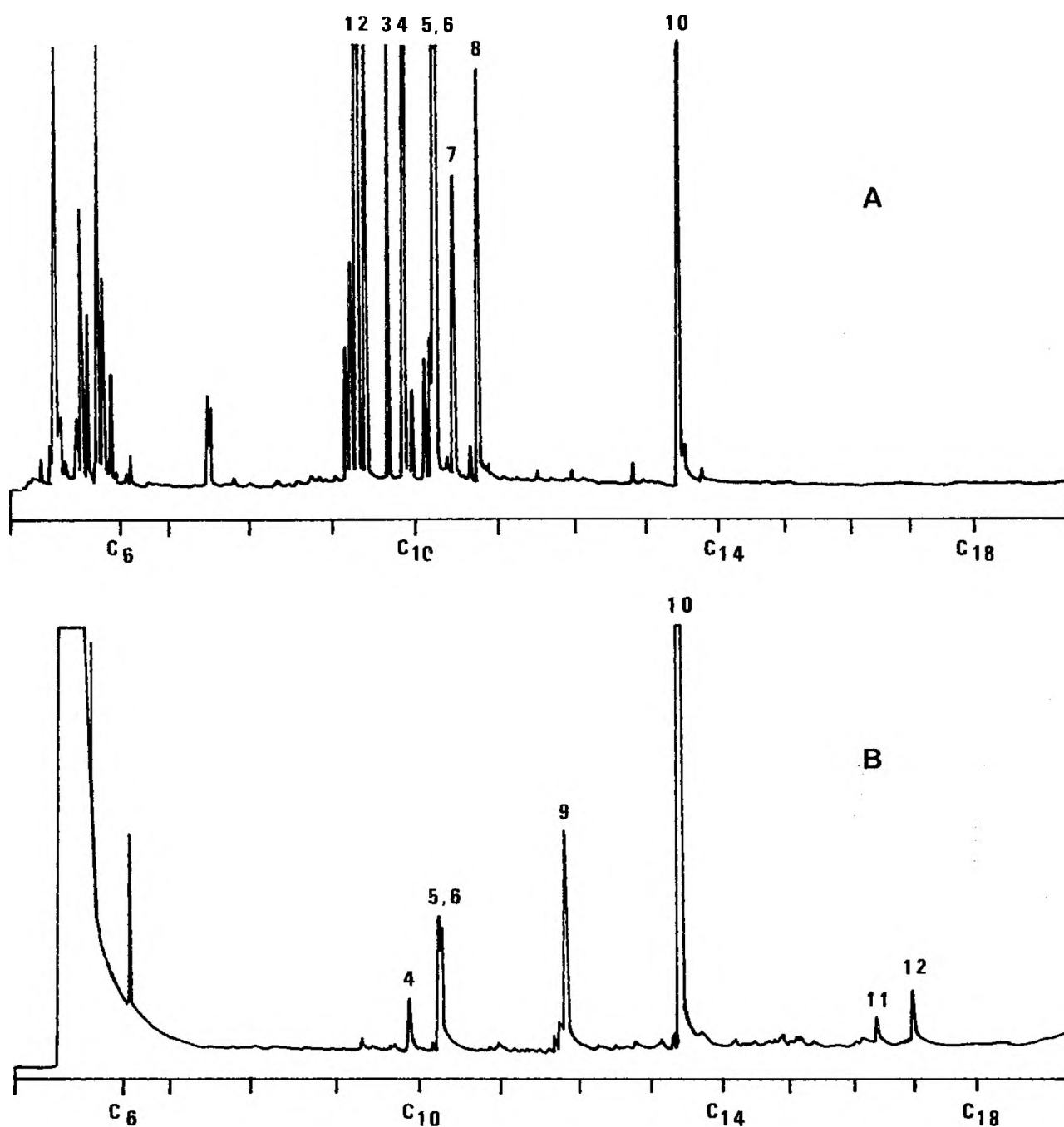
Fig. 4. Fresh lovage ( Levisticum officinale ): A. headspace; B. essential oil; 40 m OV-1 glass capillary column.
