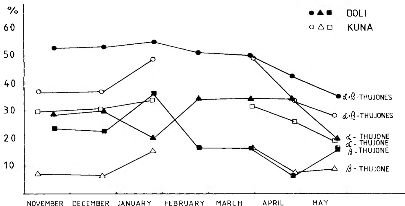
Fig. 3. Seasonal variation of \alpha - and \beta -thujone in Dalmatian sage oil from Kuna and Doli.
