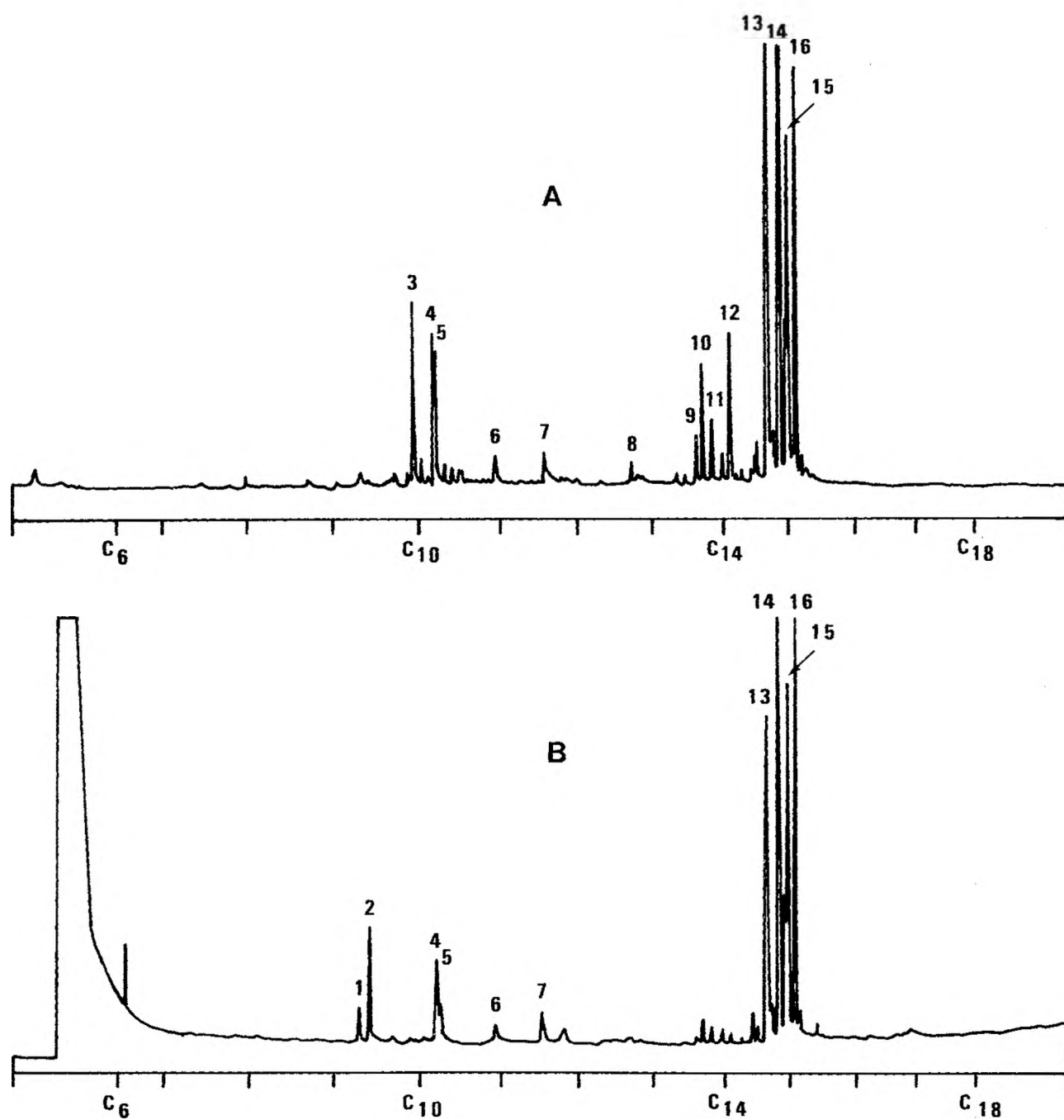
Fig. 2. Ginger powder ( Zingiber officinale ): A. headspace; B. essential oil; 40 m OV-1 glass capillary column.
