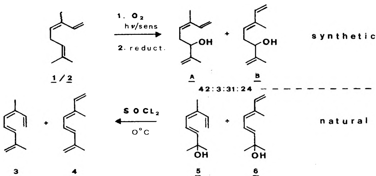
Fig. 4. Synthesis of monoterpenes newly detected in hyacinth flowers.
