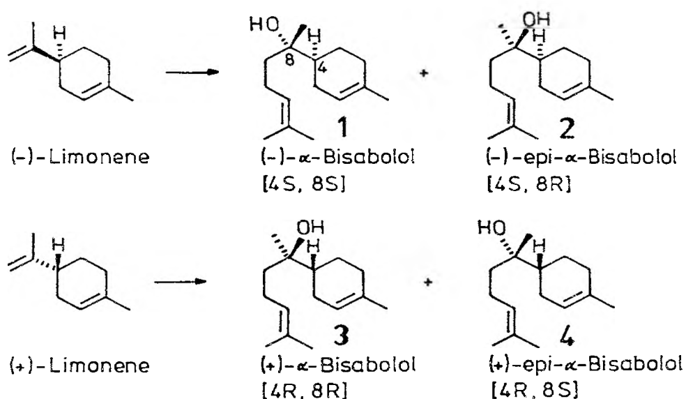
Fig. 2. Synthesis of bisabolol epimers (9).
