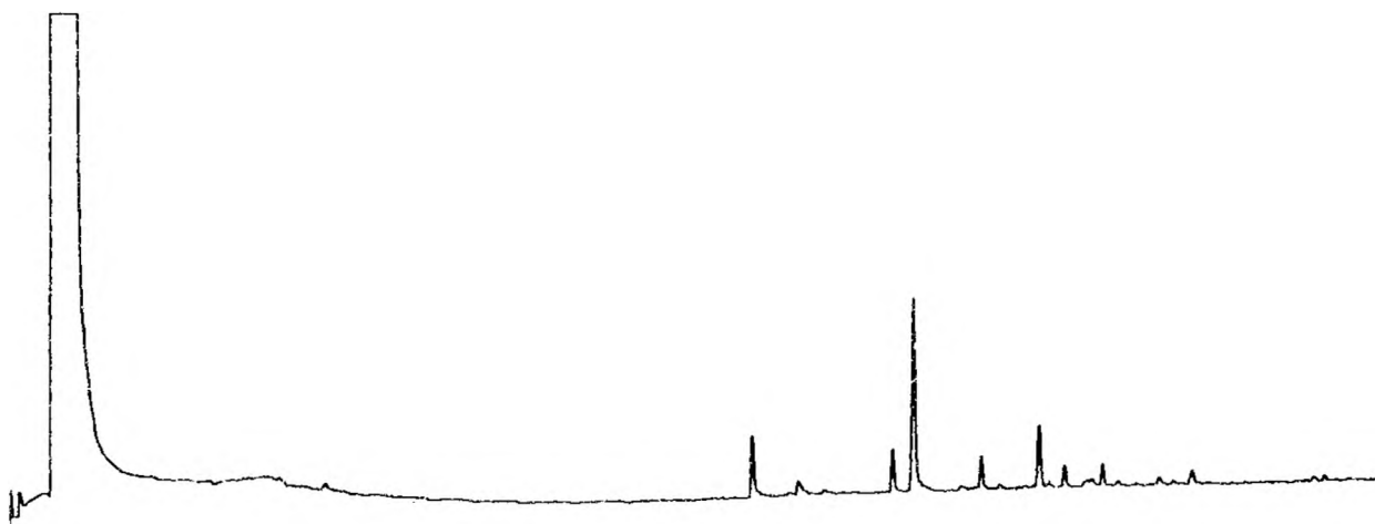
Fig.4. Soap sample with TCD.
