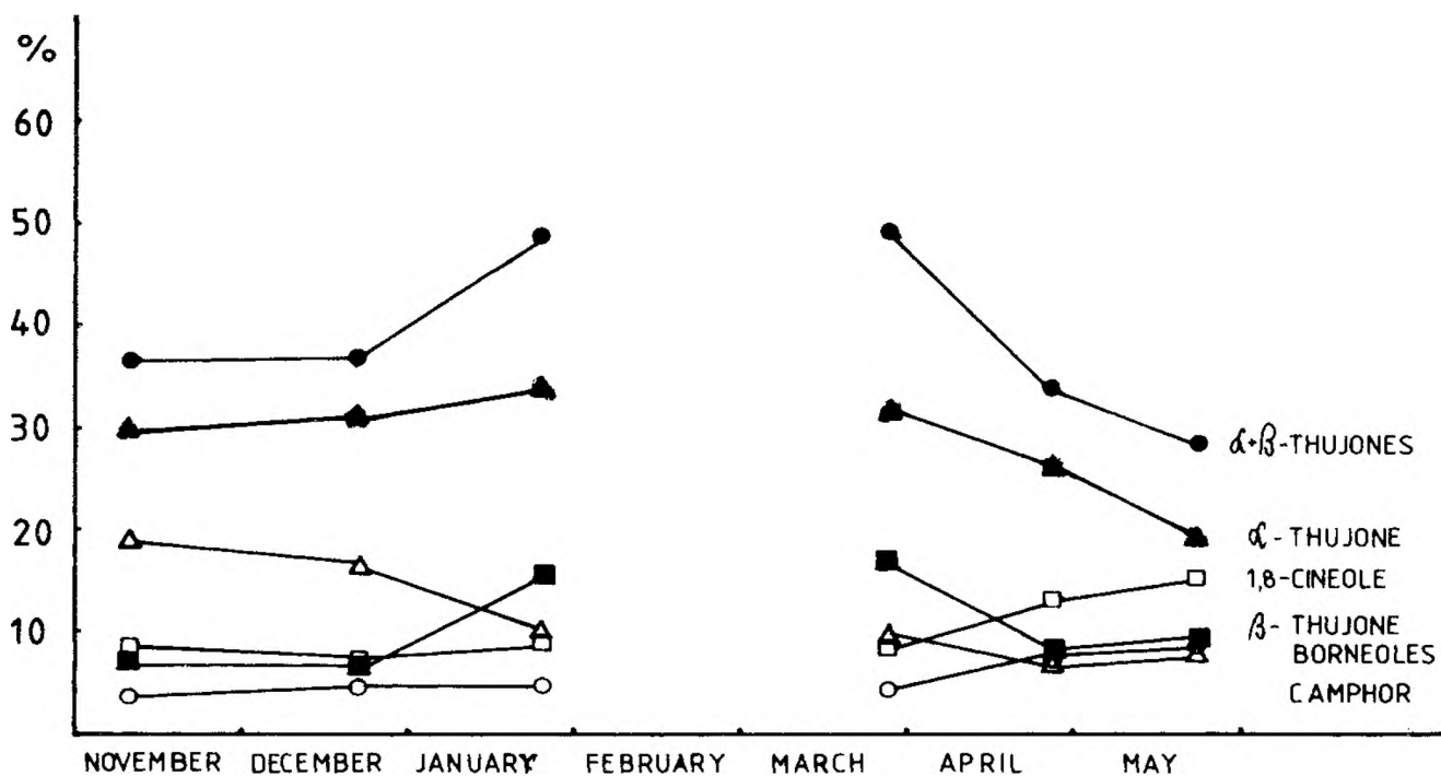
Fig. 1. Seasonal variation of the main components of Dalmatian sage oil from Kuna.
