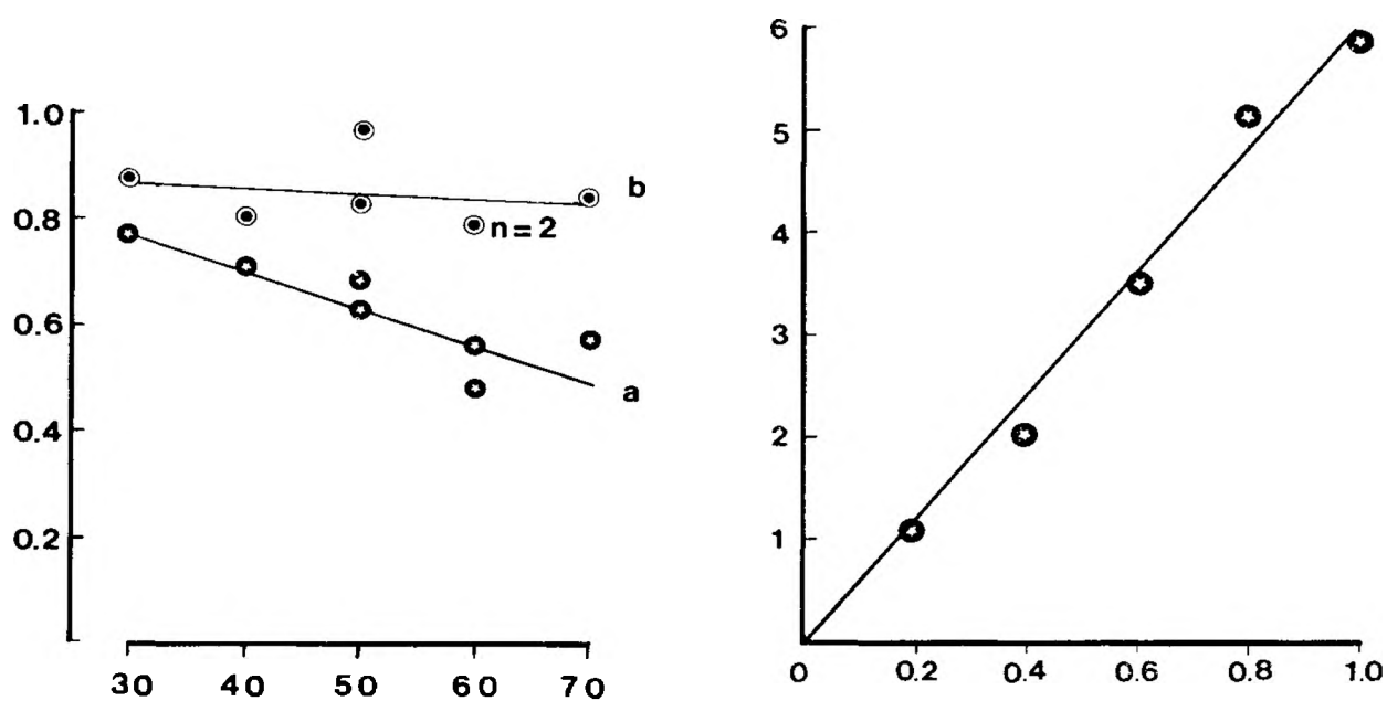
Fig. 8. The volatile oil content of thyme herb obtained by HSGC from various amounts of herb [left]: a. determined using thyme oil as external standard; b. determined using the external standard and the internal standard correction. Abscissa: amount of thyme herb in mg; ordinate: volatile oil content in percentages. The calibration curve for thyme oil [right]. Abscissa: amount of thyme oil in \mu\text{l} ; ordinate: peak area \times 10^5 .
