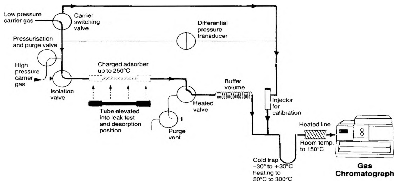
Fig. 7. The desorption process with an automatic thermal desorption system Perkin-Elmer ATD-50.
