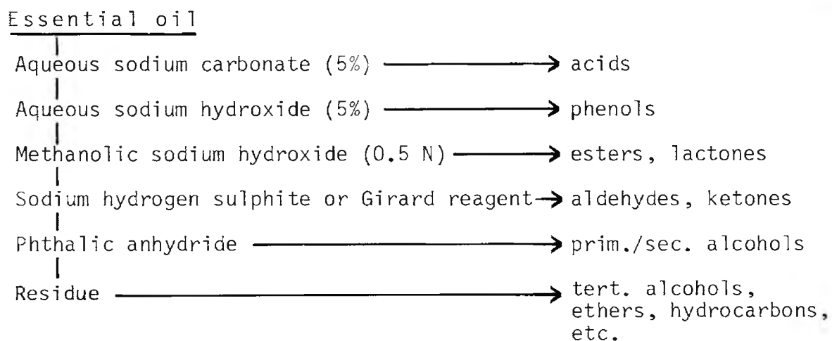
Fig. 1. Separation of an essential oil into different groups of components.
