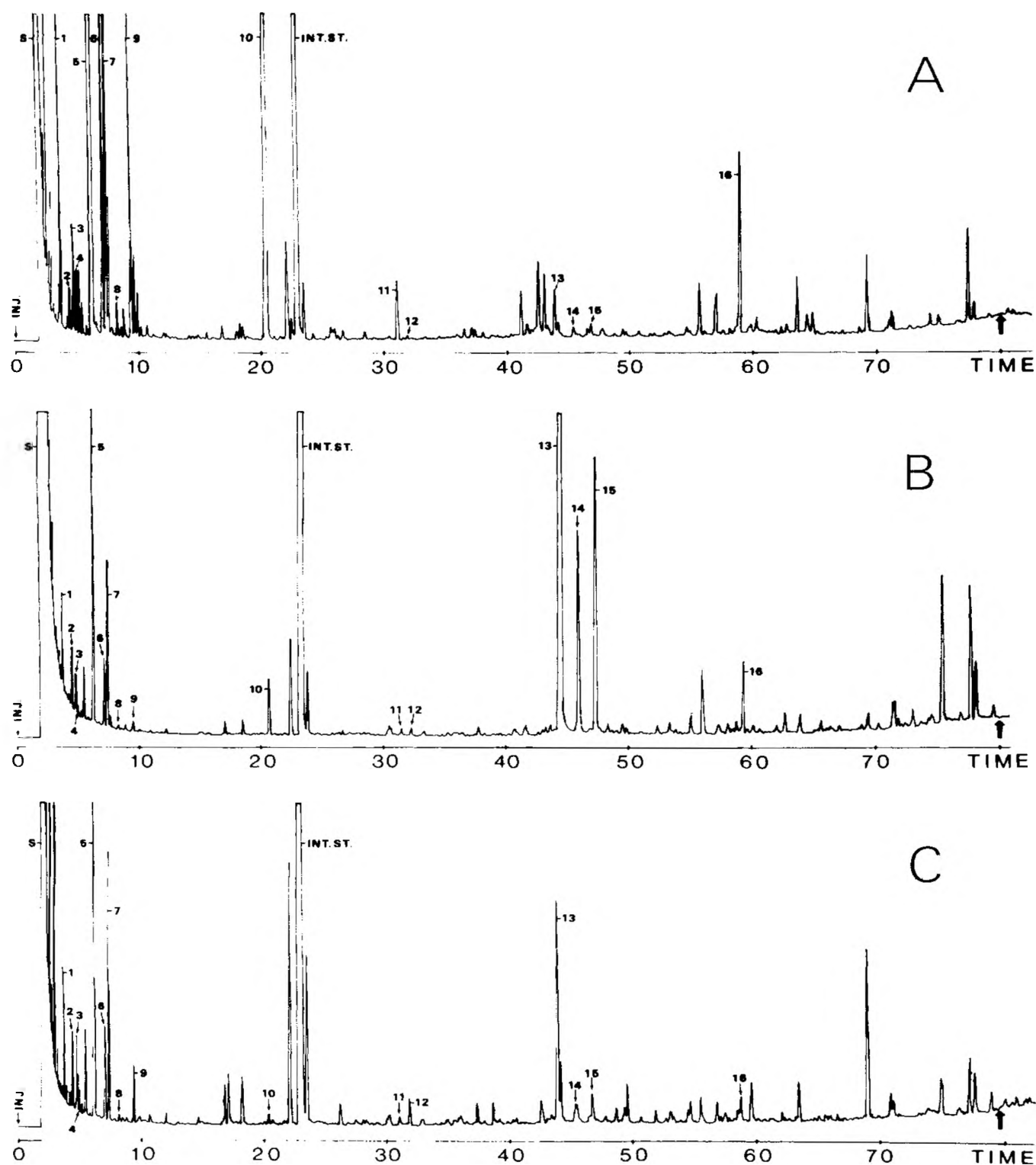
Fig. 1. Gas chromatograms of aroma concentrates isolated from fresh (A), freeze-dried (B) and air-dried (C) dill. Int. st. = internal standard (linalool); only the peaks between the solvent peak (S) and the point indicated by an arrow are included in the calculations.
