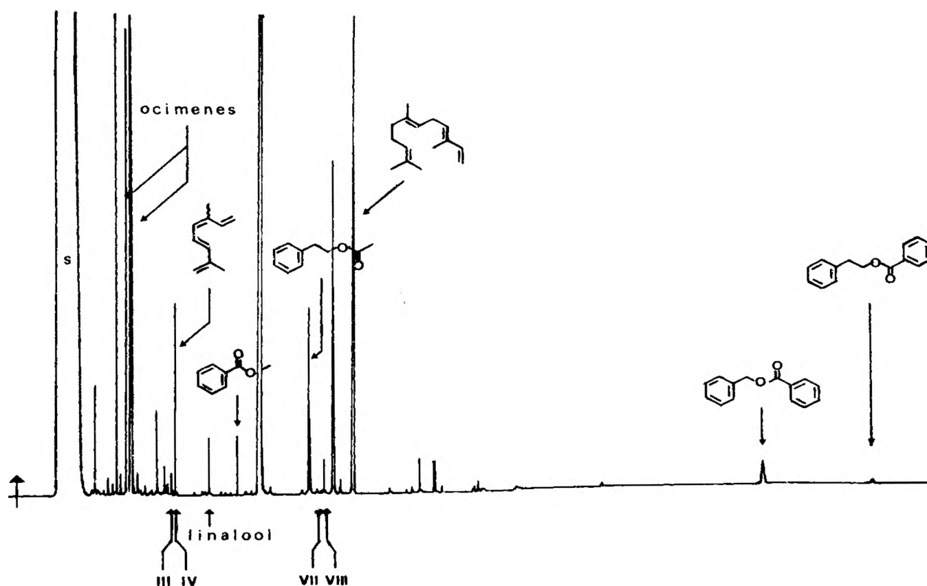
Fig. 3. Gas chromatogram of hyacinth headspace. Conditions: see Fig. 1.
