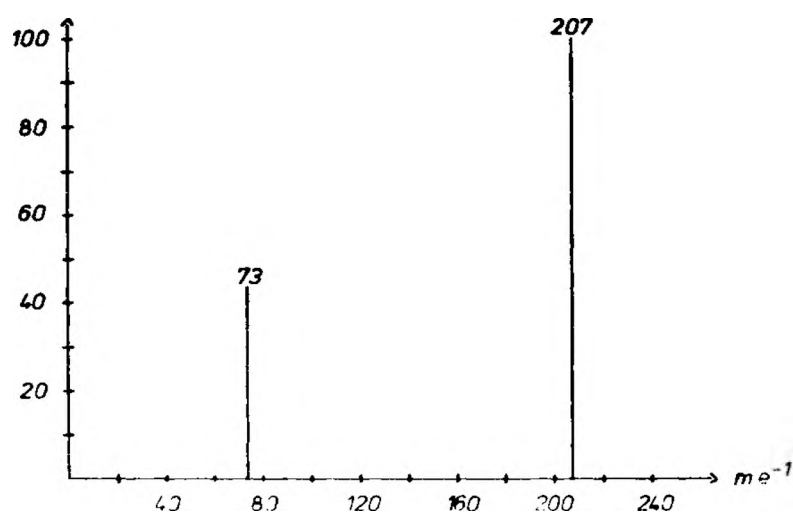
Fig. 11. Fragmentation of OV-1, three-dimensional crosslinked and chemically bonded to the Pyrex glass surface at 450°C. Ordinate: relative intensity (%).
