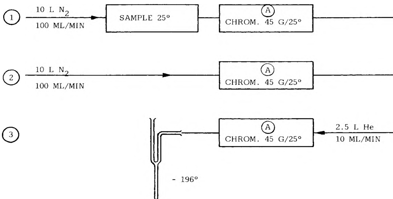
Fig. 4. Concentration of 10 l of headspace vapour. Breakthrough volumes: acetaldehyde, 24.3 l/45 g of Chromosorb 102 (25°C); water 4.9 l/45 g of Chromosorb 102 (25°C). Desorption volume: acetaldehyde 1.8 l/45 g of Chromosorb 102 (150°C).
