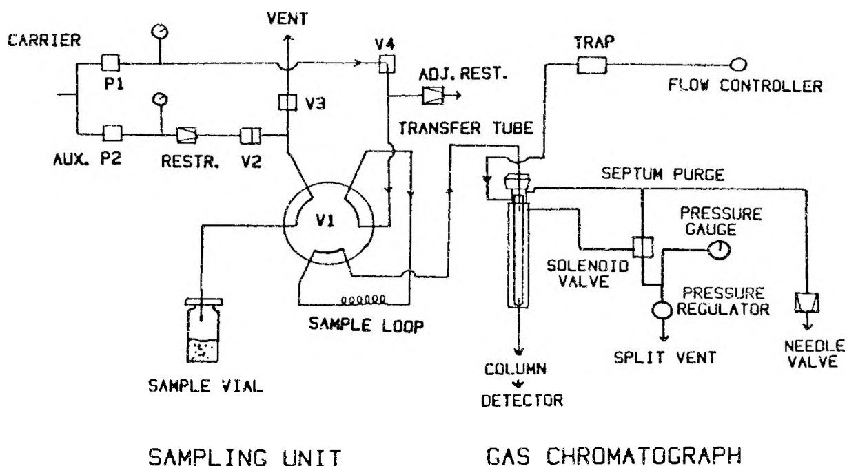
Fig.2. Scheme of the analysis system in the sampling mode.
