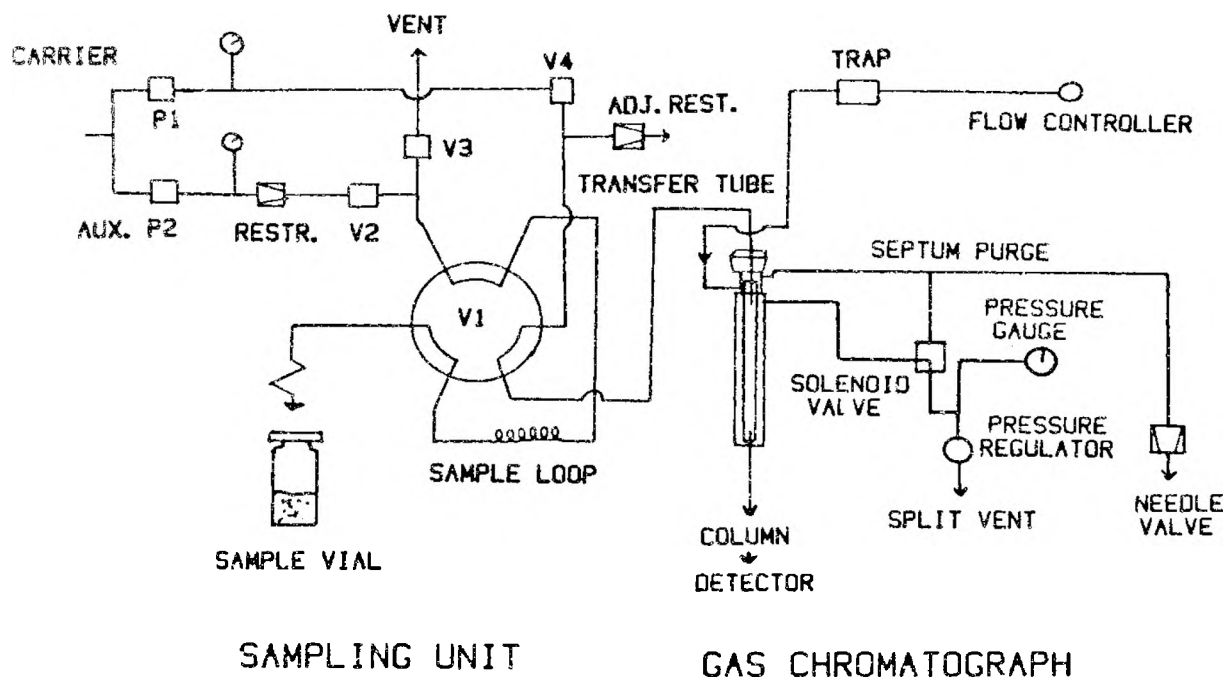
Fig.1. Scheme of the analysis system in the standby mode.
