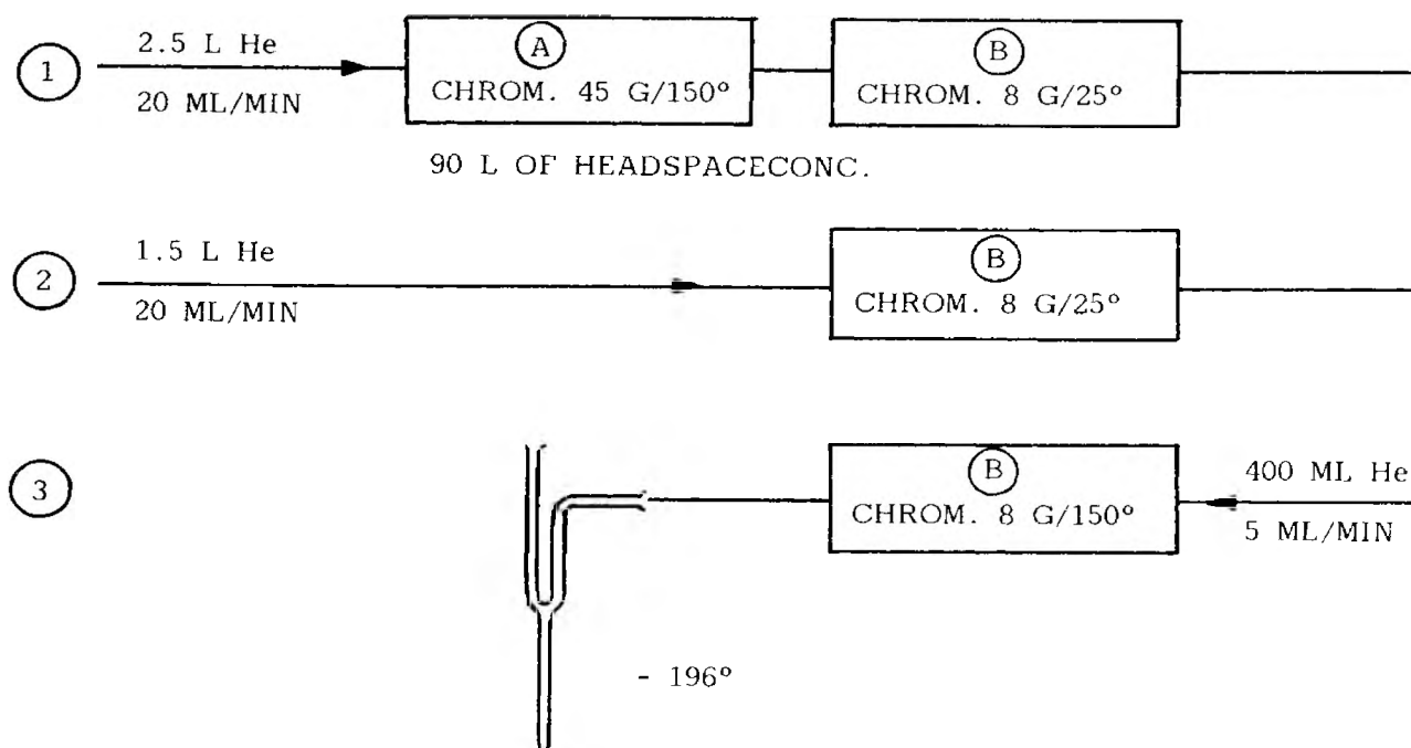
Fig. 6. Water-free collection of 90 l of headspace volatiles. Breakthrough volume of acetaldehyde (Chromosorb 102): 4.3 l/8 g (25° C). Desorption volumes: 1.8 l/45 g (150°C); 32 ml/8 g (150°C).
