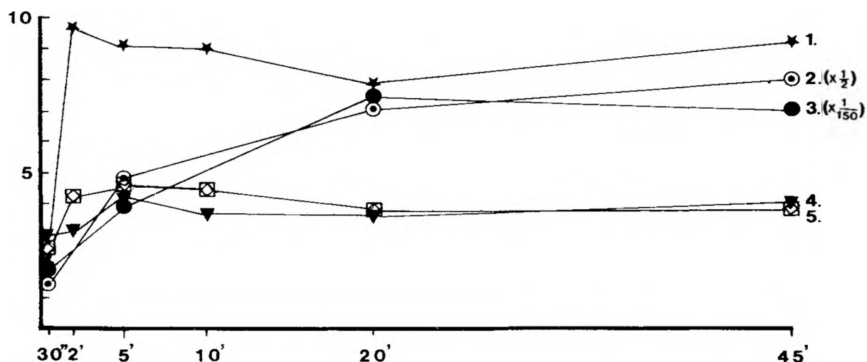
Fig. 5. The effect of equilibration period on the peak areas of some terpenes in solid samples, in HSGC analyses at a bath temperature of 150°C: 1. oxygenated monoterpenes in thyme herb; 2. bisabolol oxide A in chamomile flowerheads; 3. \alpha -bisabolol in chamomile flowerheads; 4. MTHC in thyme herb; 5. sesquiterpenes in thyme herb. Abscissa: equilibration period; ordinate: peak area \times 10^4 .
