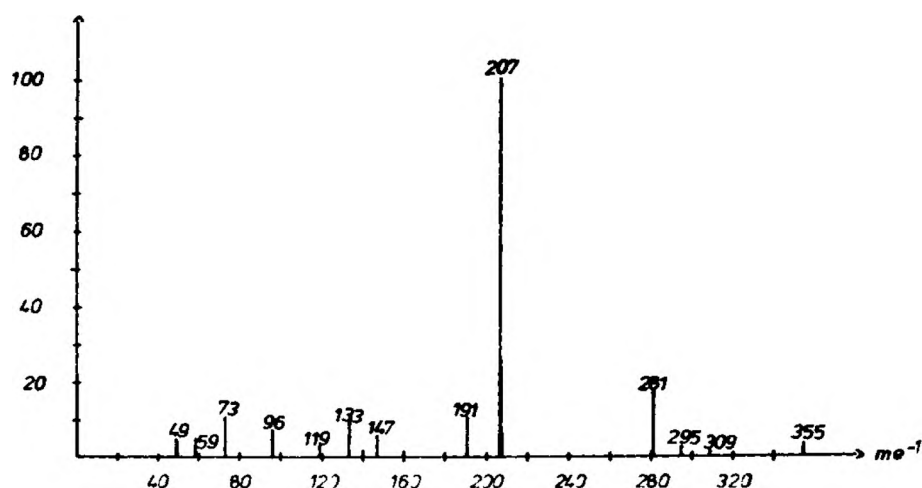
Fig. 10. Fragmentation of OV-1, three-dimensional crosslinked on Pyrex glass at 375°C. Ordinate: relative intensity (%).
