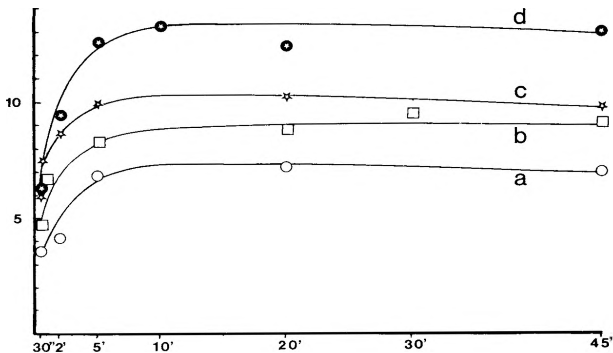
Fig. 3. The effect of equilibration period on the peak area of thymol in HSGC analyses at various temperatures: a = 60°C; b = 90°C; c = 120°C; d = 150°C. Abscissa: equilibration period; ordinate: peak area \times 10^4 .
