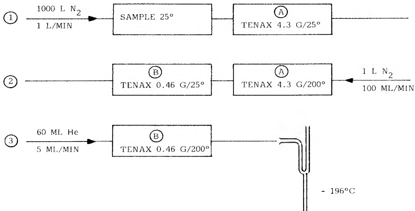
Fig. 8. Concentration of 1000 l of headspace vapour. Breakthrough volumes: water, 258 ml/4.3 g of Tenax GC (25°C); ethyl butyrate, 1075 l/4.3 g of Tenax GC (25°C); ethyl butyrate, 115 l/0.46 g of Tenax GC (25°C). Desorption volume: ethyl butyrate, 100 ml/4.3 g of Tenax GC (200°C).
