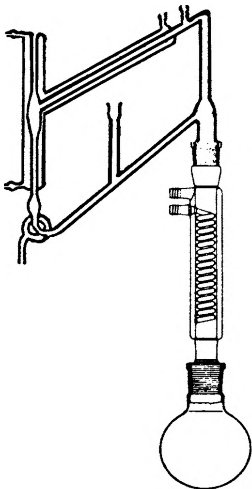
Fig. 1. Schematic drawing of the apparatus used to study the influence of the pH of the distillation medium on the stability of various compounds.
