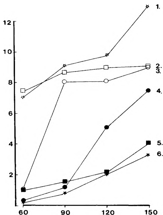
Fig. 1. The effect of bath temperature on the peak areas of some terpenes: 1. thymol; 2. mixture of MTHC; 3. \alpha -bisabolol; 4. \alpha -bisabolol in chamomile flowerheads; 5. MTHC in thyme herb; 6. thymol in thyme herb. Abscissa: bath temperature ( ^{\circ}\text{C} ); ordinate: peak area \times 10^4 .
