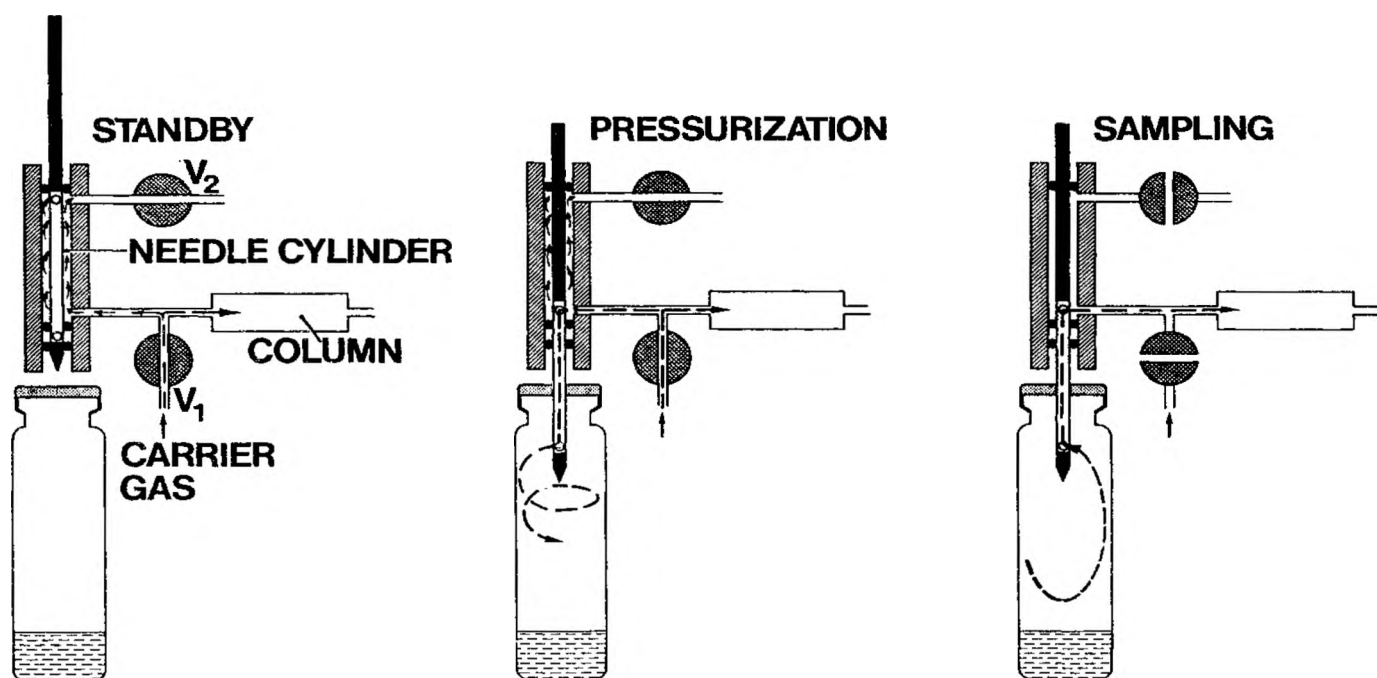
Fig. 1. Balanced pressure sampling with the Perkin-Elmer HS-100 Automatic Headspace Sampler.
