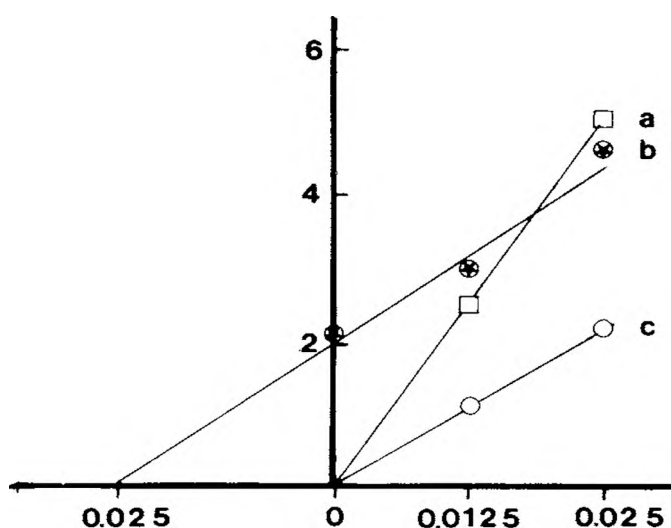
Fig. 10. Calibration curves for the single run HSGC determination of the volatile oil amount in thyme herb: a. thymol as external standard; b. thymol added to the matrix (thyme herb); c. thymol added to the matrix after first having distilled off the volatile oil. Abscissa: added amount of thymol in mg; ordinate: peak area \times 10^4 .
