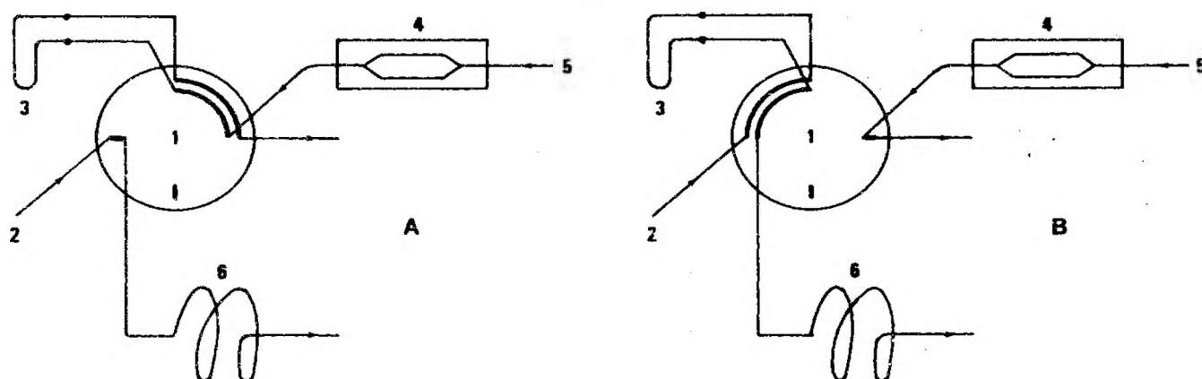
Fig. 1. Desorption-injection system: A. desorption and collection of the volatiles in a cold trap; B. injection by heating the cold trap. 1. two-position, six-port, high temperature injection valve (Valco Instruments, Houston, U.S.A.); 2. carrier gas, Helium, 4 ml/min; 3. cold trap (in liquid air); 4. desorption oven and adsorption tube; 5. sweeping gas, Helium, 10-12 ml/min; 6. glass capillary column.
