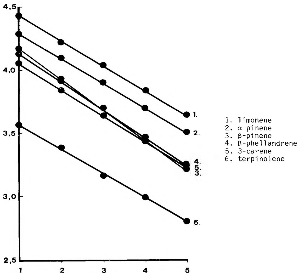
Fig. 15. MHE-HSGC analysis of some monoterpene hydrocarbons. Abscissa: number of extractions; ordinate: log peak area.
