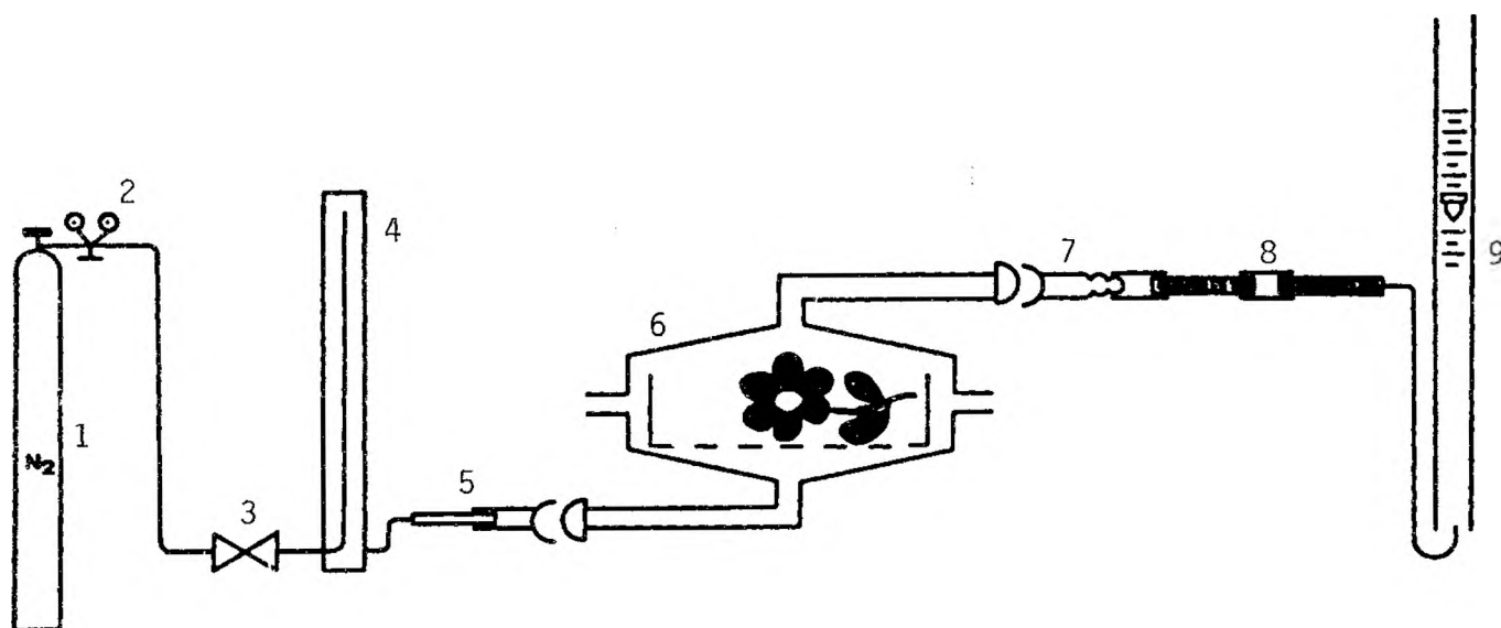
Fig. 2. Headspace apparatus (schematic). 1. Nitrogen cylinder; 2. reducing valve; 3. needle valve; 4. tower with molecular sieves; 5. connection; 6. vessel with grate; 7. connection; 8. charcoal filters (two); 9. rotameter.
