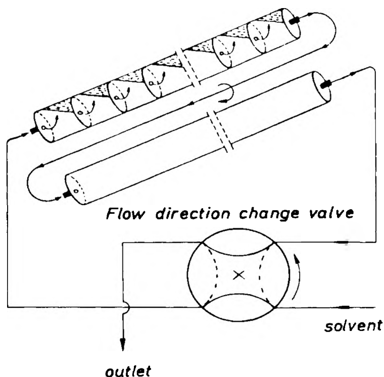
Fig. 12. Flow scheme of the RLCC apparatus.
