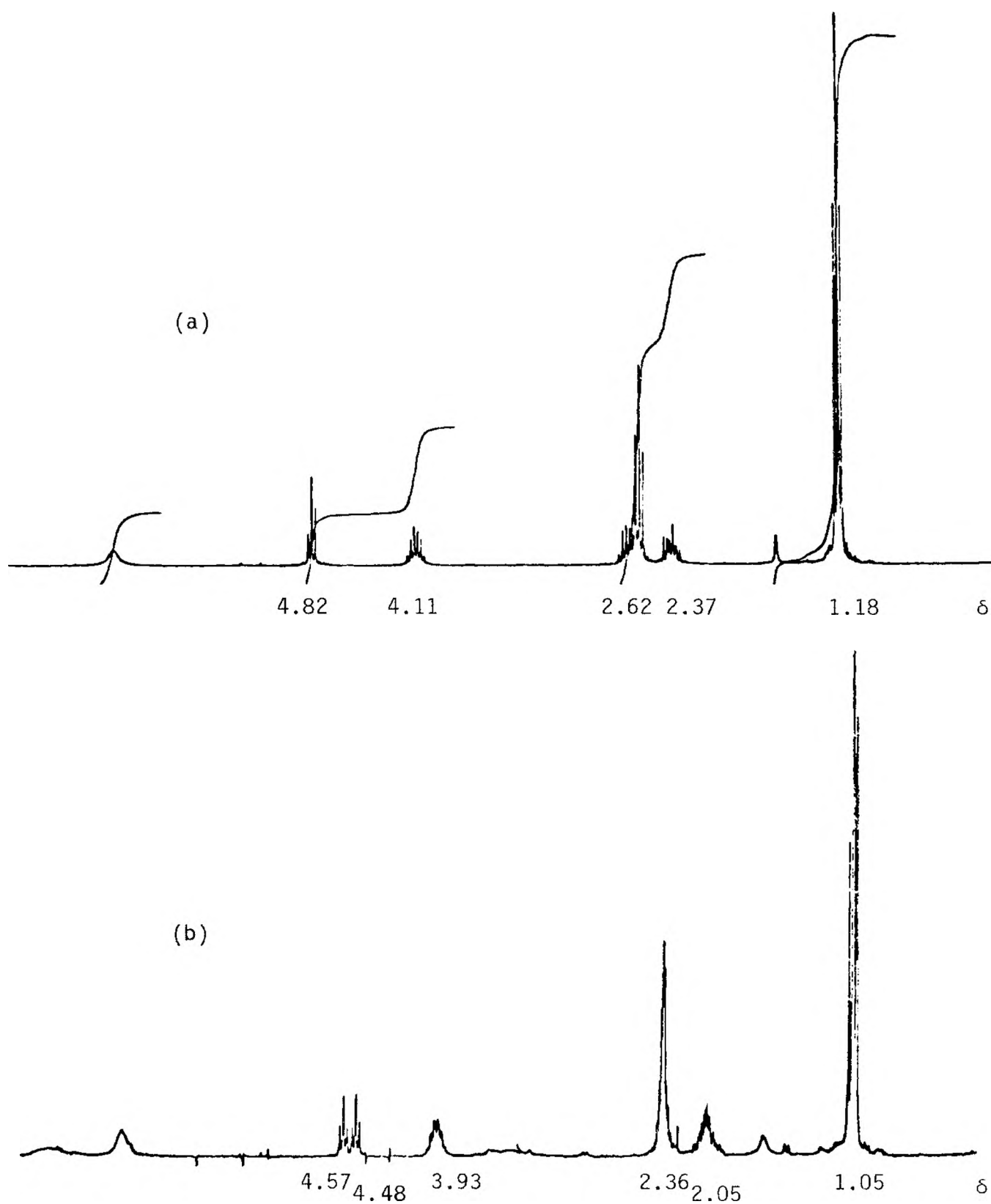
Fig. 1. NMR spectra of enantiomerically pure 4-isopropylaminocarbonyl- \gamma -butyrolactone. (a) neat; (b) in presence of TFAE
