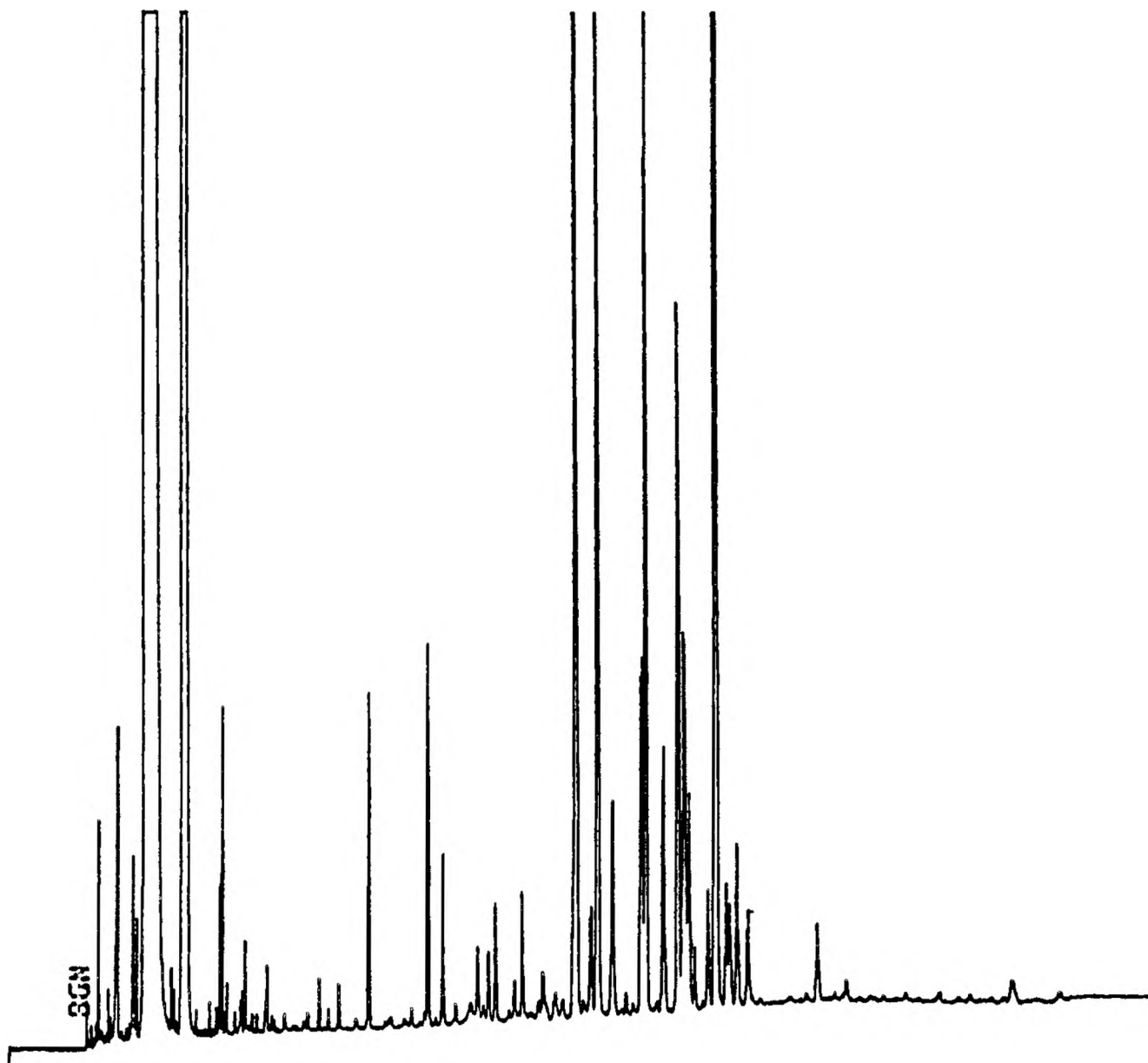
Fig. 8. Analysis of perfume headspace by adsorption on Tenax GC. Perkin-Elmer ATD-50; column, fused silica capillary coated with Perma-phase DMS (dimethyl silicon); temperature program, 50-200°C (4°C/min); sampling: 15 min passive sampling with Tenax GC packed ATD-50 tube over a perfume bottle.
