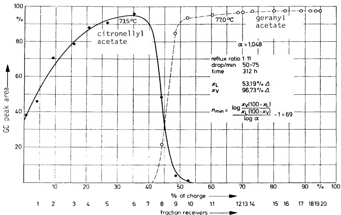
Fig. 3. Separation of citronellyl acetate and geranyl acetate by means of a 'Spaltrohr' distillation column (reproduced with the permission of Fischer Labor- u. Verfahrenstechnik, Meckenheim, FRG).
