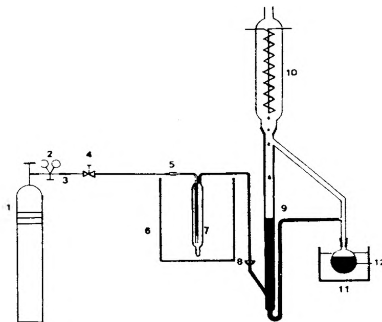
Fig. 3. Schematic drawing of the apparatus used to isolate the volatiles from plant extracts by gas phase stripping (10): 1. inert gas supply; 2. pressure reducer; 3. charcoal filter; 4. flow regulator; 5. connection with Teflon shrinking tube; 6. water bath (30°C); 7. sample container with plant extract; 8. connection by ground-ball-socket joint; 9. extraction chamber; 10. reflux condenser (-30°C); 11. water bath (30°C); 12. flask with Freon 11.
