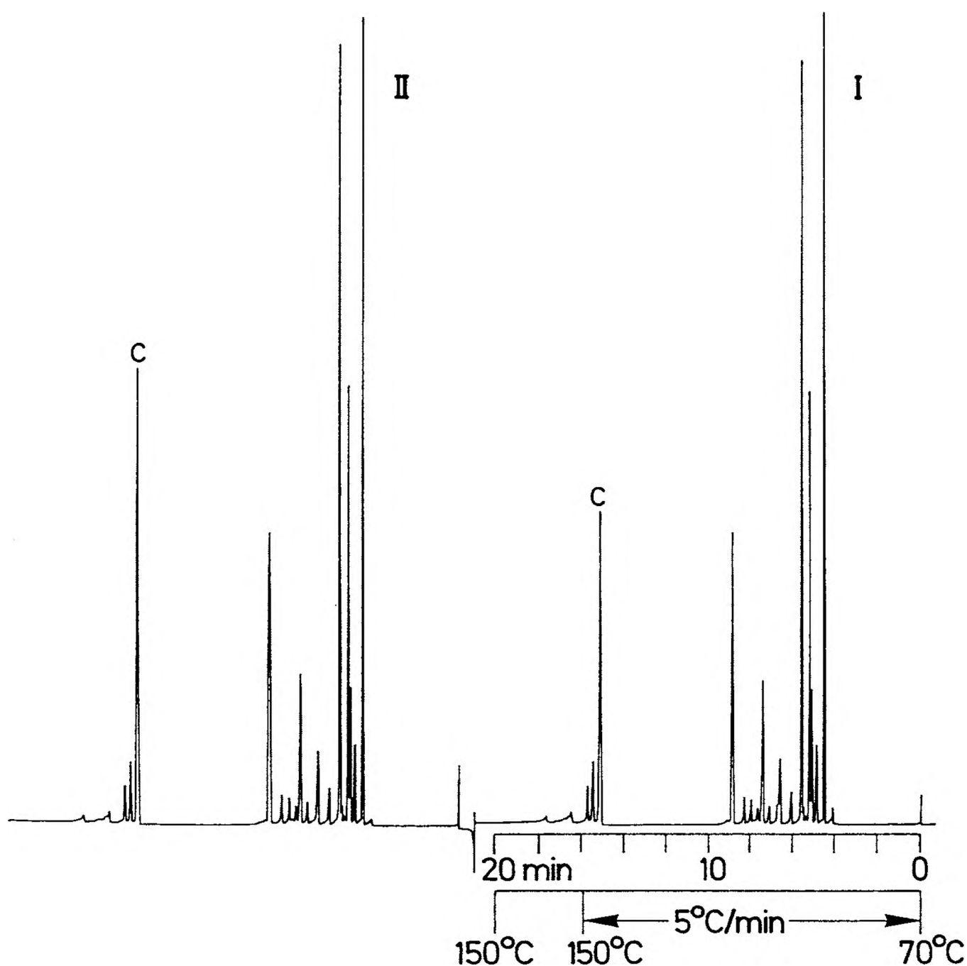
Fig. 4. Quantitative headspace analysis of 1.1% camphor (C) in massage cream by the technique of standard addition. Perkin-Elmer Sigma 2, HS-6; column, glass capillary, coated with Carbowax 20M; split injection; chromatogram I, 1 g sample at 80°C; chromatogram II, 1 g sample + 5 mg camphor.
