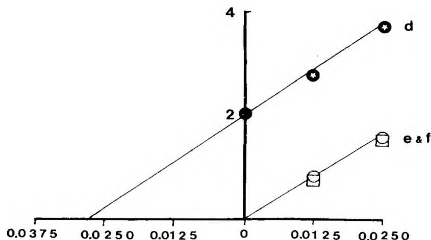
Fig. 11. Calibration curves for the MHE-HSGC determination of the volatile oil amount in thyme herb: d. thymol added to the matrix (thyme herb); e. thymol as external standard; f. thymol added to the matrix after first having distilled off the volatile oil. Abscissa: added amount of thymol in mg; ordinate: peak area \times 10^5 .
