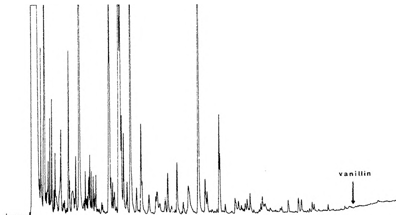
Fig. 11. Gas chromatogram of vanilla bean headspace. Conditions: glass capillary column, 50 m x 0.33 mm, coated with UCON HB 5100; temperature program, room temperature (15 min), 50°C (15 min) then 50-180°C (3°C/min); carrier gas, Helium; injection, 0.5 \mu l on cold column.
