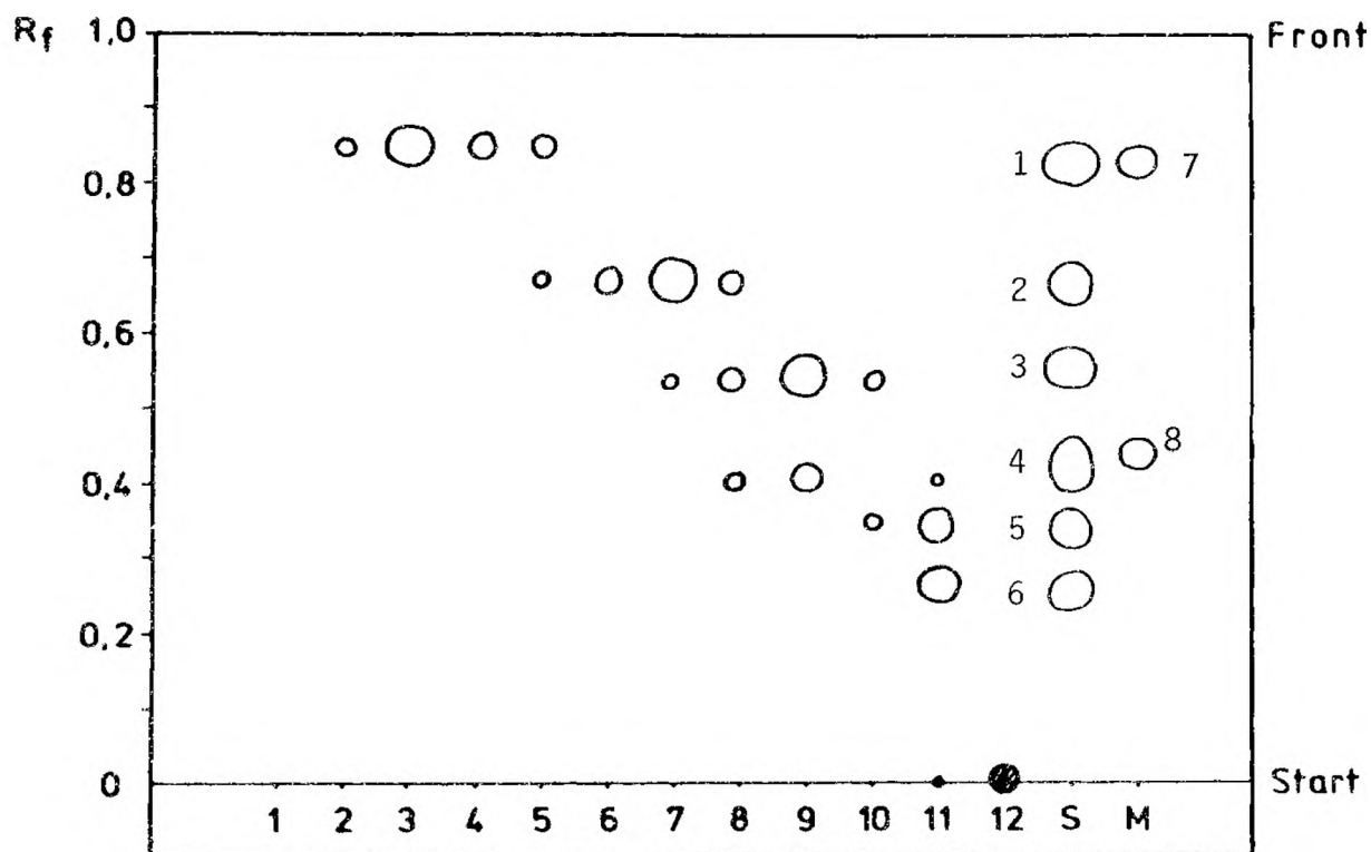
Fig. 4. TLC (silica gel/n-pentane at -18^\circ\text{C} ) of the 12 fractions obtained by silica gel dry-column chromatography with n-pentane at -18^\circ\text{C} . S and M = sesqui- and monoterpene hydrocarbons: 1 = \alpha -copaene; 2 = \delta -elemene; 3 = \beta -elemene; 4 = \beta -caryophyllene; 5 = \beta -bisabolene; 6 = \alpha -humulene; 7 = \alpha -pinene; 8 = limonene.
