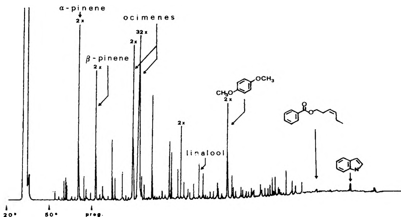
Fig. 9. Gas chromatogram of lilac headspace. Conditions: glass capillary column, 50 m x 0.33 mm, coated with UCON HB 5100; temperature program, 50°C (9 min) then 50-180°C (3°C/min); carrier gas, Helium; injection, 0.5 µl on cold column.
