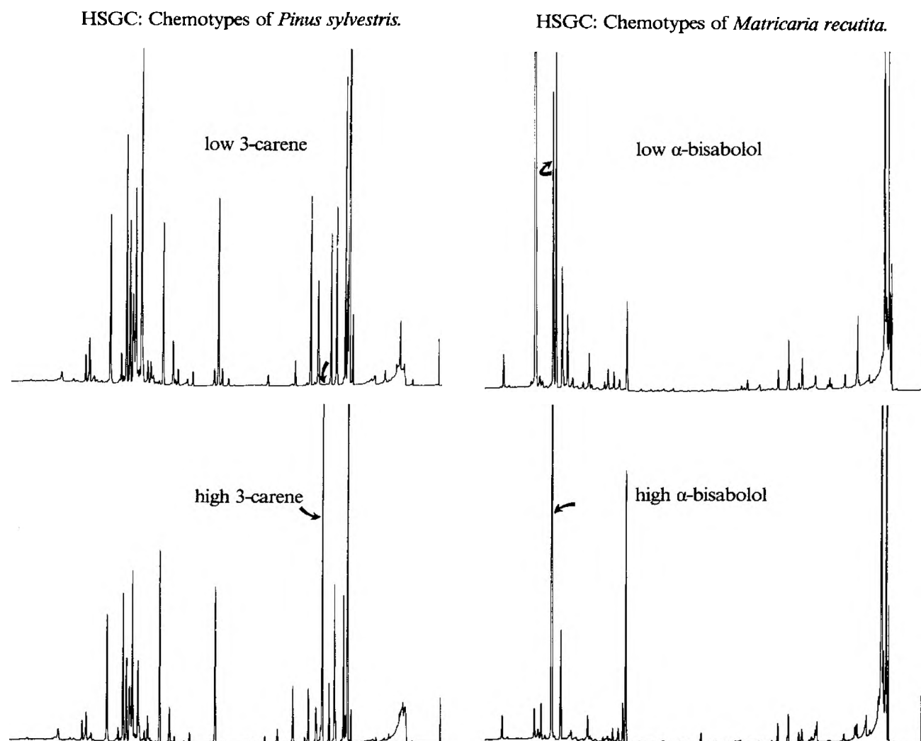
Fig. 6. Chromatograms obtained by HSGC showing two chemotypes of Pinus sylvestris (left) and two chemotypes of Matricaria recutita (right).
