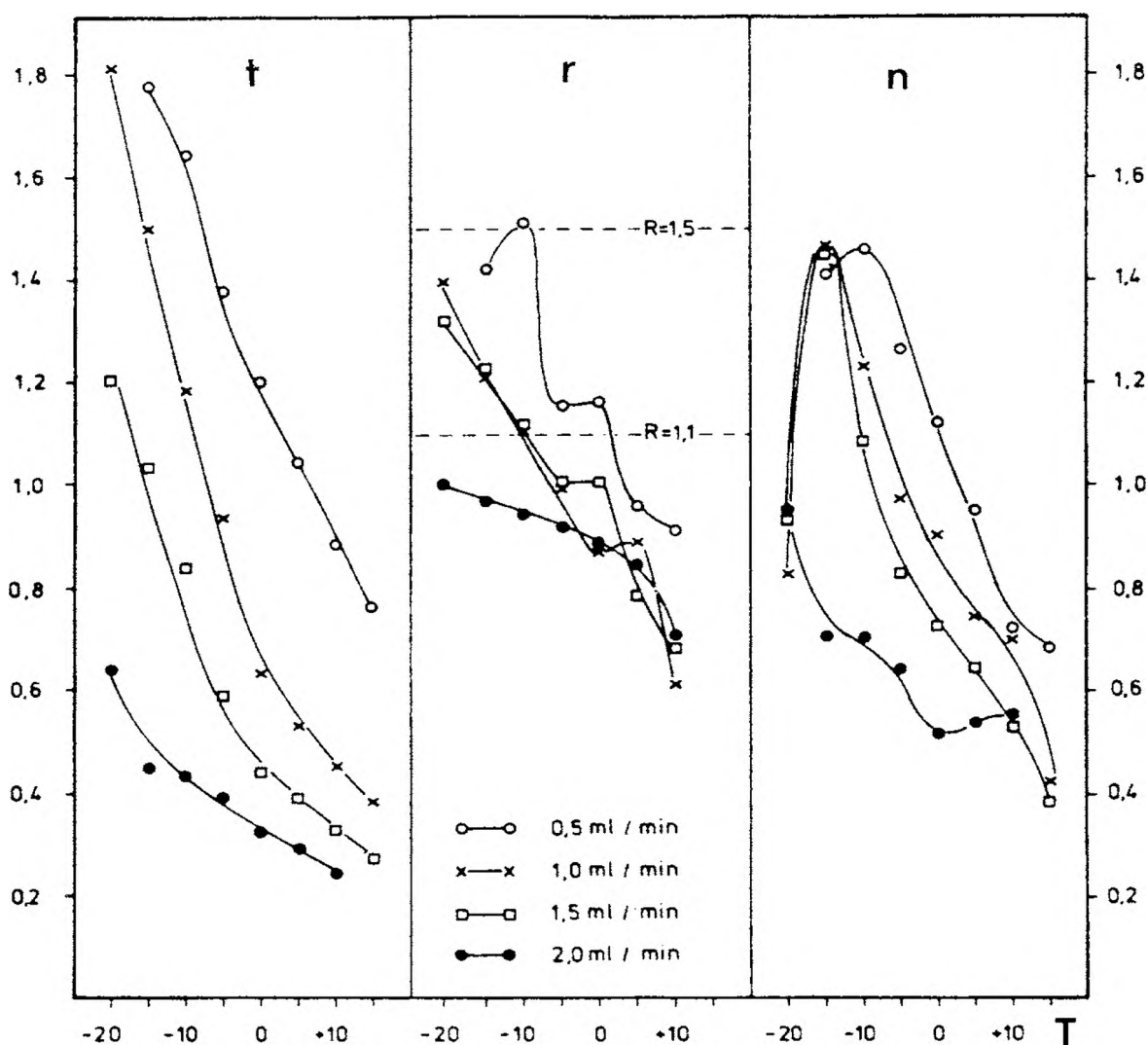
Fig. 9. Analysis time t , resolution r and plate number n versus column temperature T in adsorption HPLC of terpene hydrocarbons on silica gel with n -pentane.
