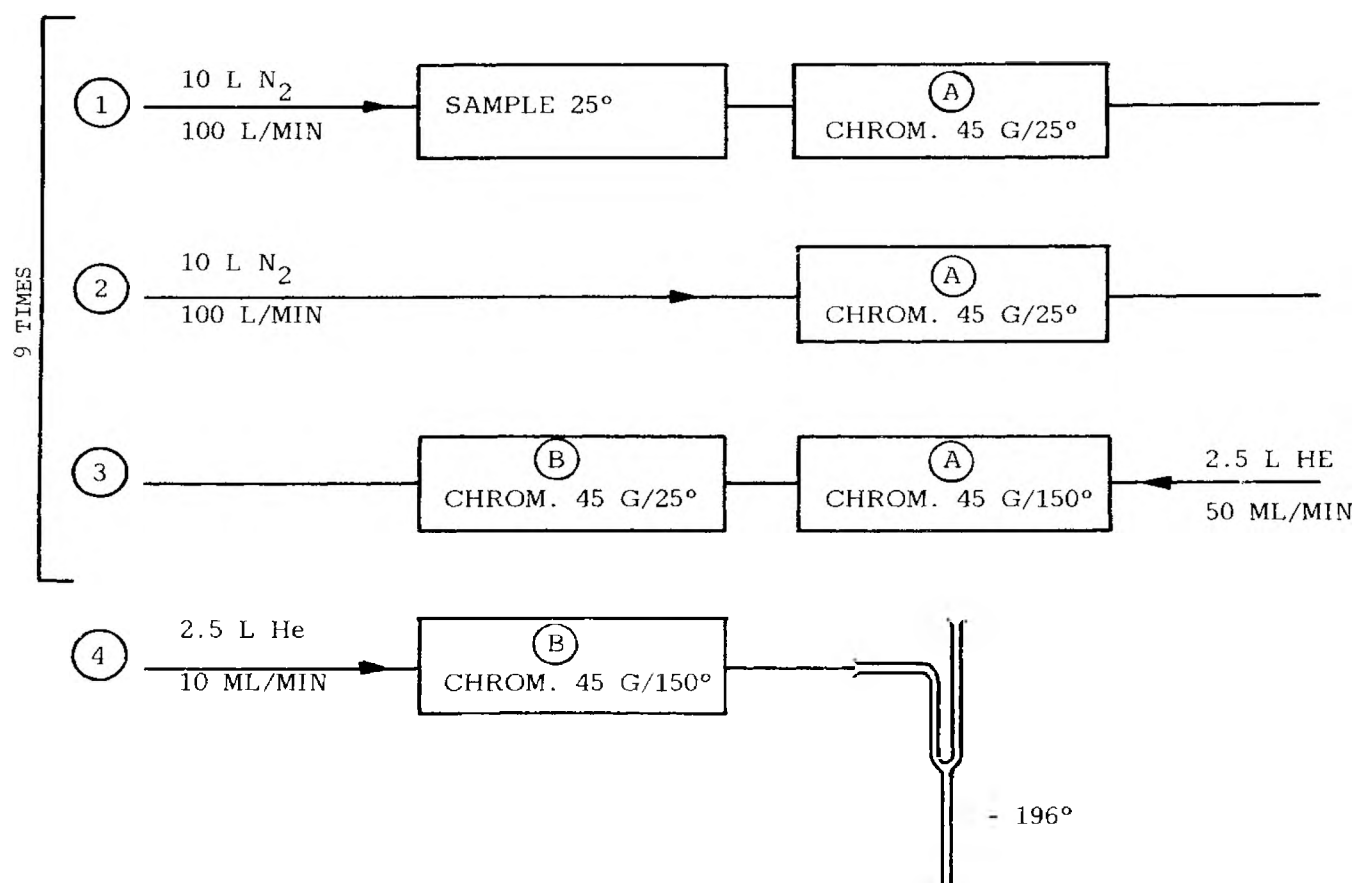
Fig. 5. Concentration of 90 l of headspace vapour. Breakthrough volumes and desorption volume: see Fig. 4.
