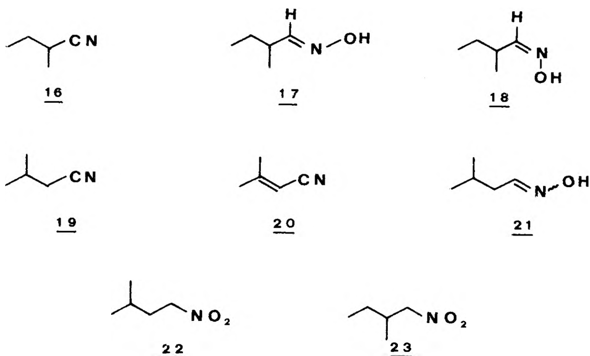
Fig. 7. Constituents of Lonicera species.
