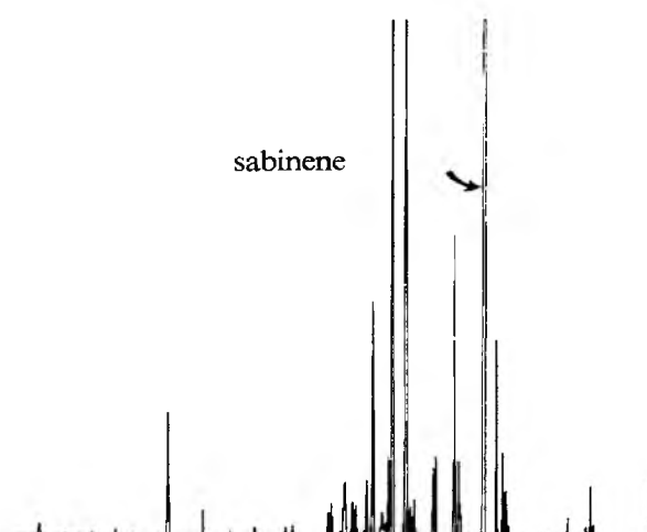
HSGC: Chemotypes of Tanacetum vulgare .
