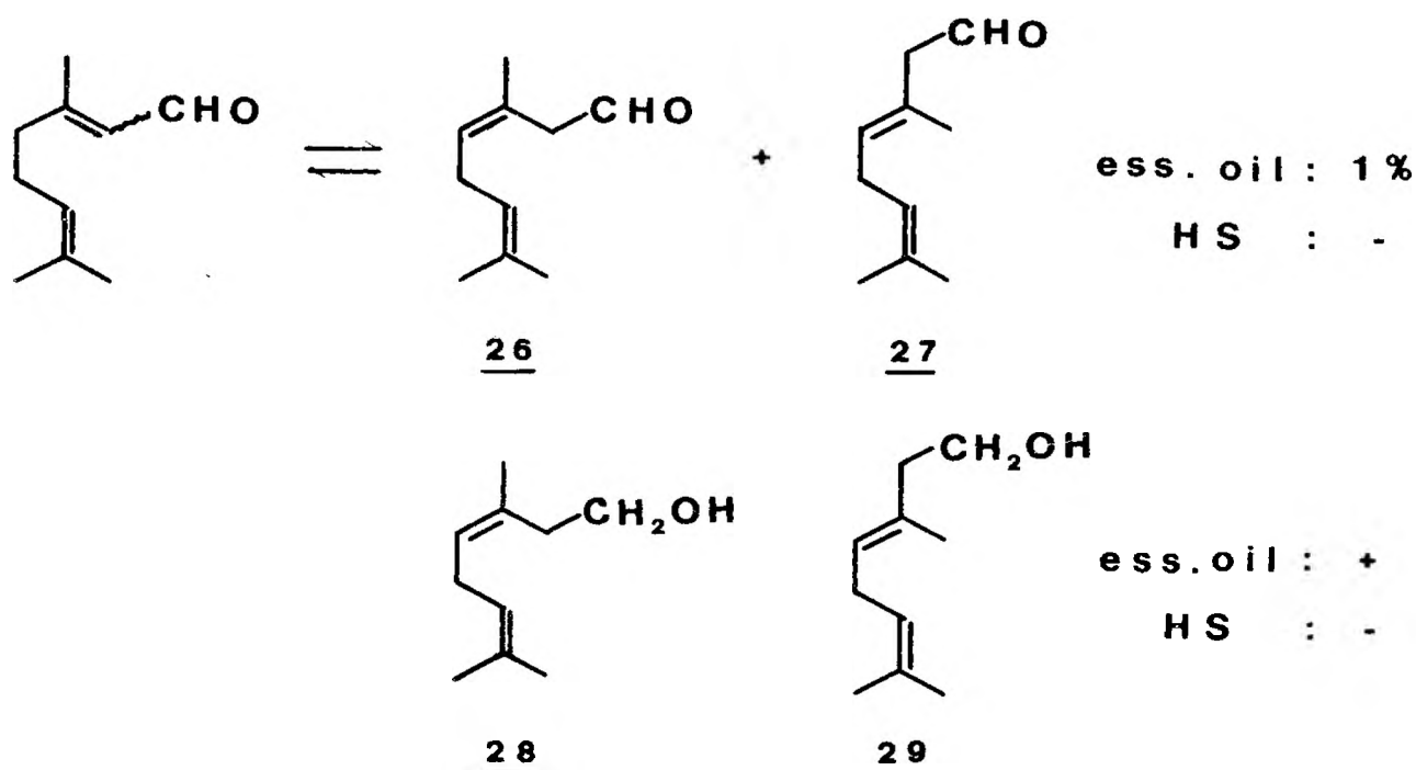
Fig. 10. Isomeric citral derivatives present in verbena oil and absent in headspace (HS) of flowering verbena herb.
