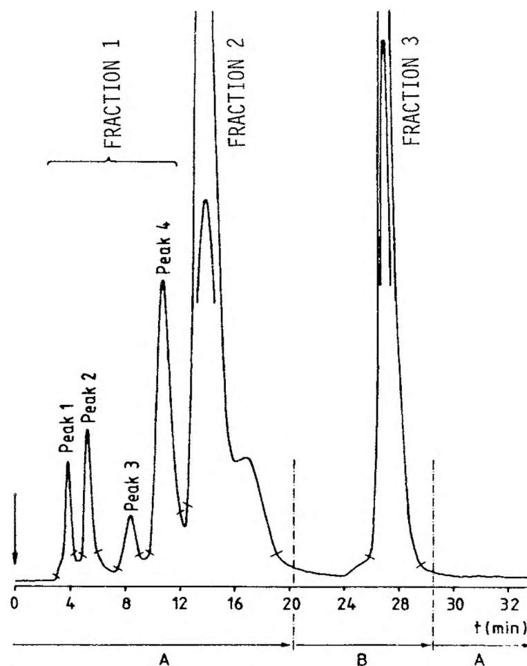
Fig. 8. HPLC fractionation of an essential oil at a flow rate of 4 ml/min. Other conditions, see Fig. 7.
