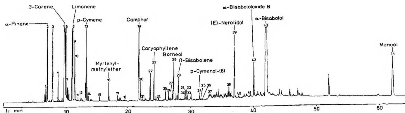
Fig. 1. Gas chromatogram of the essential oil of Salvia stenophylla .
