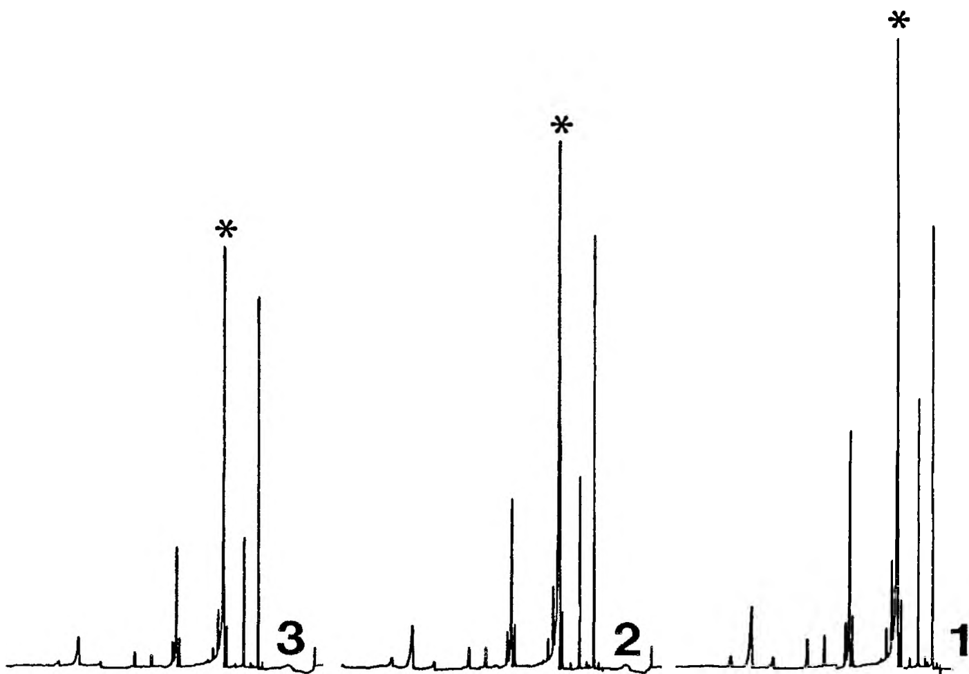
Fig. 5. Determination of 73 ppm (w/w) trans-1,2-dichloroethylene in coffee powder by multiple headspace extraction (MHE). Perkin-Elmer Sigma 2000, HS-100; column, fused silica (50 m x 0.32 mm) coated with SE-54; 70°C isothermal; carrier gas, Helium; split injection; sample, 474 mg coffee + 100 \mu\text{l} water (displacer), 30 min at 80°C.
