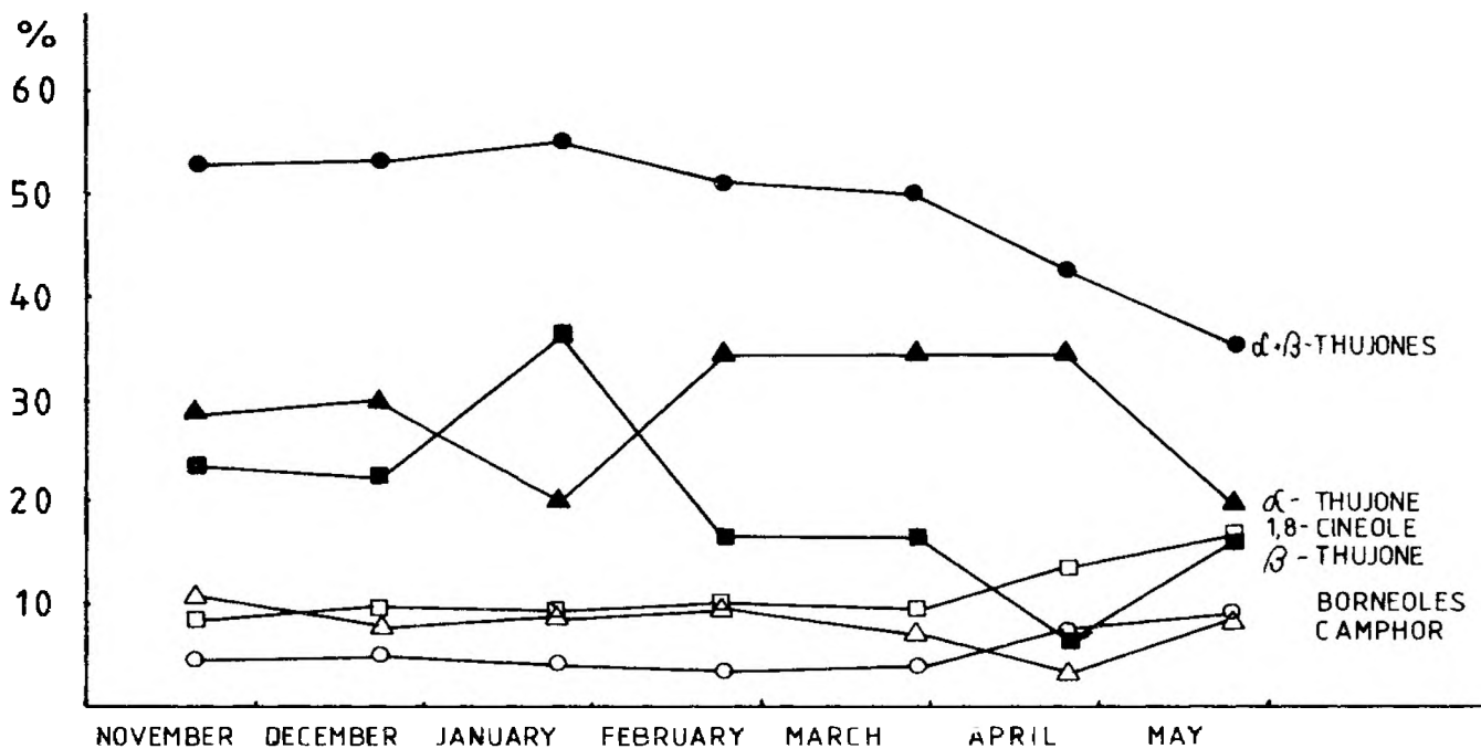
Fig. 2. Seasonal variation of the main components of Dalmatian sage oil from Doli.
