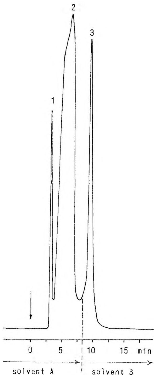
Fig. 7. HPLC fractionation of an essential oil at a flow rate of 8 ml/min.
