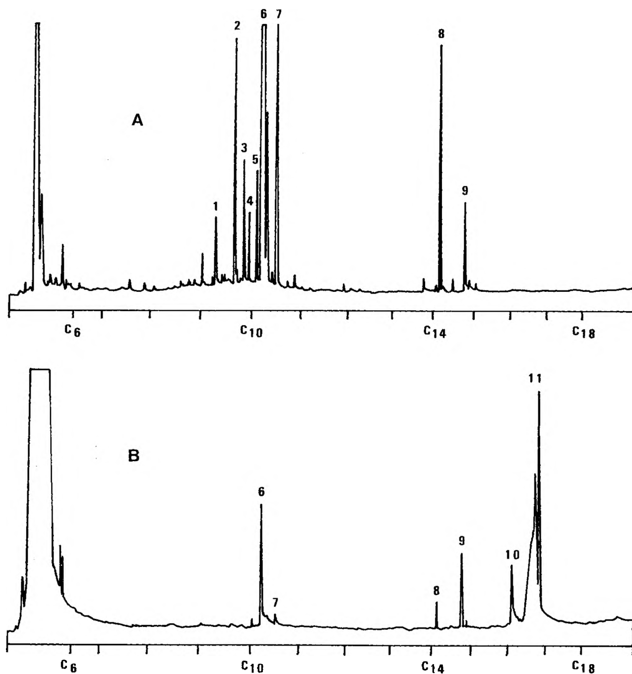
Fig. 3. Fresh celery ( Apium graveolens cv dulce ): A. headspace; B. essential oil; 40 m OV-1 glass capillary column.
