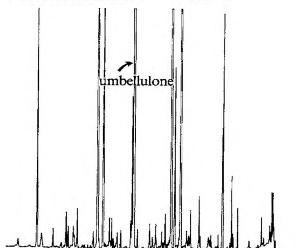
Fig. 7. Chromatograms obtained by HSGC showing four chemotypes of Tanacetum vulgare .
