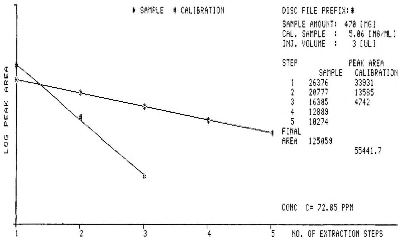
Fig. 6. Quantitative determination of 73 ppm (w/w) trans-1,2-dichloroethylene in coffee powder by a five-step MHE analysis (see Fig. 5) with linear regression calculation.
