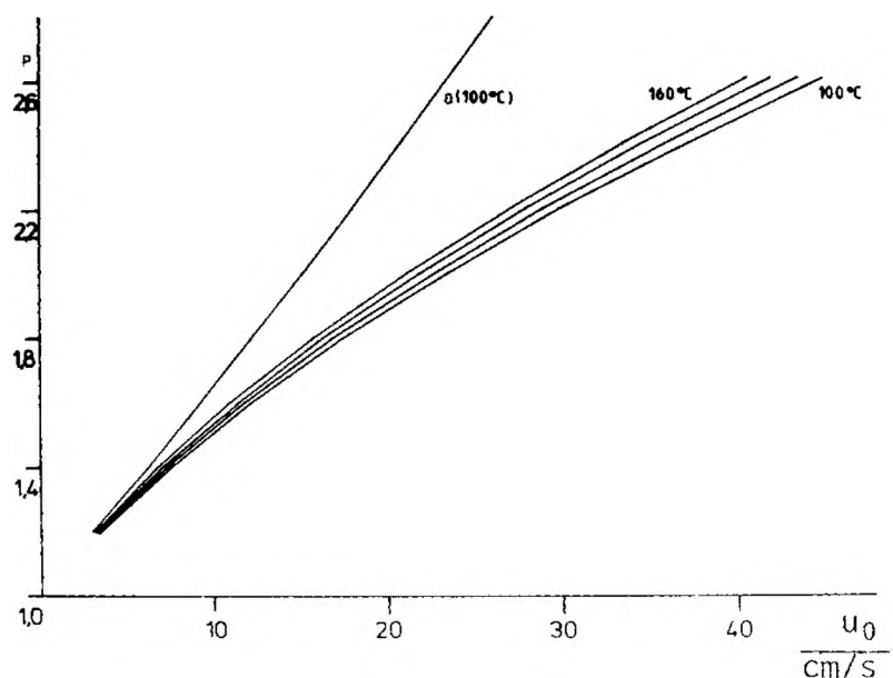
Fig. 9. Relation between gas velocity at the end of the column and pressure at different temperatures. Fused silica capillary WG-11 column (47 m x 0.22 mm i.d.) carrier gas, Nitrogen.
