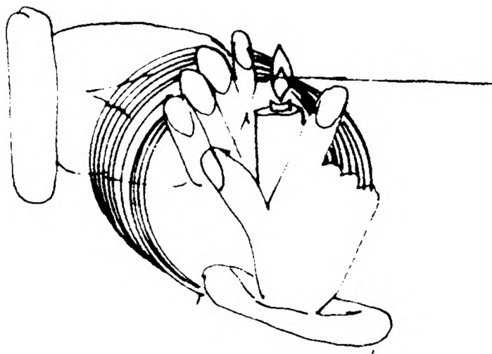
Fig. 3. Position for bending up glass capillary ends.
