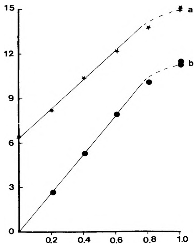
Fig. 8. The volatile oil content of thyme herb obtained by HSGC from various amounts of herb [left]: a. determined using thyme oil as external standard; b. determined using the external standard and the internal standard correction. Abscissa: amount of thyme herb in mg; ordinate: volatile oil content in percentages. The calibration curve for thyme oil [right]. Abscissa: amount of thyme oil in \mu\text{l} ; ordinate: peak area \times 10^5 .
