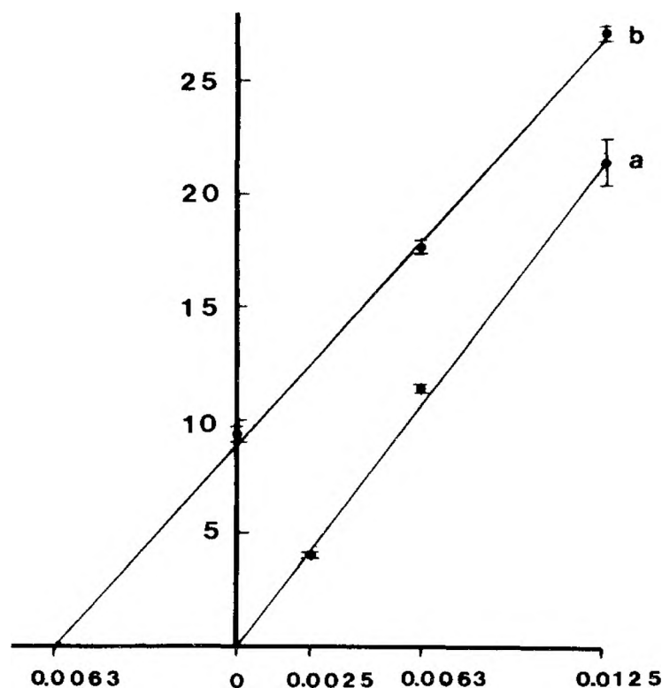
Fig. 14. Determination of the amount of \alpha -bisabolol in a commercially available chamomile preparation: a. \alpha -bisabolol added to an artificial matrix, ethanol-water, N = 3 ; b. \alpha -bisabolol added to a chamomile preparation, N = 6 . Abscissa: added amount of \alpha -bisabolol in mg; ordinate: peak area \times 10^3 .
