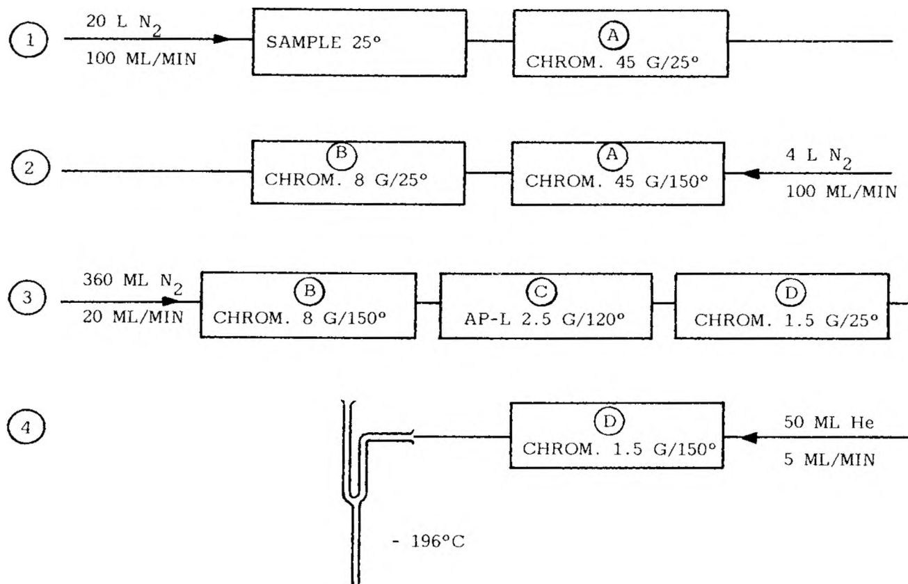
Fig. 9. Hydrocarbon-free collection of headspace volatiles of essential oils. Breakthrough volumes (in addition to those mentioned in Figs. 4 and 6): \alpha -pinene, 400 ml/2.5 g of Apiezon-L (120°C); acetaldehyde, 800 ml/1.5 g of Chromosorb 102 (25°C). Desorption volume: acetaldehyde, 50 ml/1.5 g of Chromosorb 102 (150°C)
