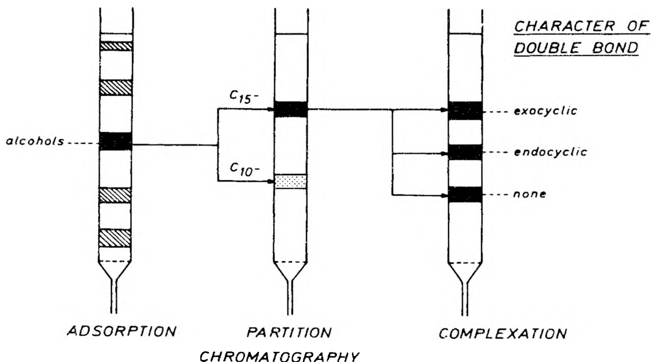
Fig. 5. Separation of sesquiterpene alcohols from an Artemisia oil by using different types of columns in series (12).
