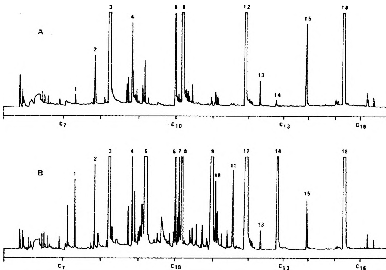
Fig. 6. Intact apples ( Malus domestica cv Golden Delicious): A. headspace; 150 m SE-52 glass capillary column; B. headspace after 24 h incubation with pentanoic acid vapours at 17°C; 150 m SE-52 glass capillary column; C. essential oil; 40 m OV-1 glass capillary column. 1. Propyl acetate 10. Hexyl propionate 2. 2-Methylpropyl acetate 11. Pentyl 2-methylbutyrate 3. Butyl acetate 12. Butyl hexanoate + hexyl butyrate 4. 3-Methylbutyl acetate 13. Hexyl 2-methylbutyrate 5. Pentyl acetate 14. Hexyl pentanoate 6. Butyl butyrate 15. Hexyl hexanoate 7. Pentyl propionate 16. \alpha -Farnesene 8. Hexyl acetate 9. Pentyl butyrate
