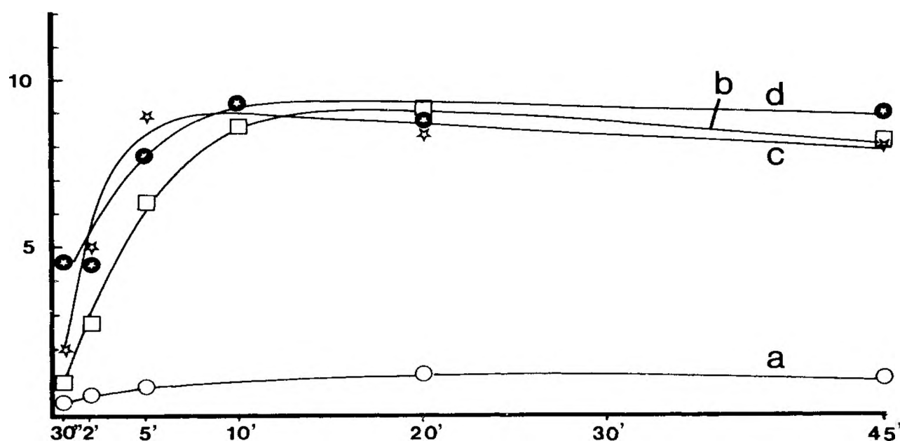
Fig. 4. The effect of equilibration period on the peak area of \alpha -bisabolol in HSGC analyses at various temperatures: a = 60°C; b = 90°C; c = 120°C; d = 150°C. Abscissa: equilibration period; ordinate: peak area \times 10^4 .
