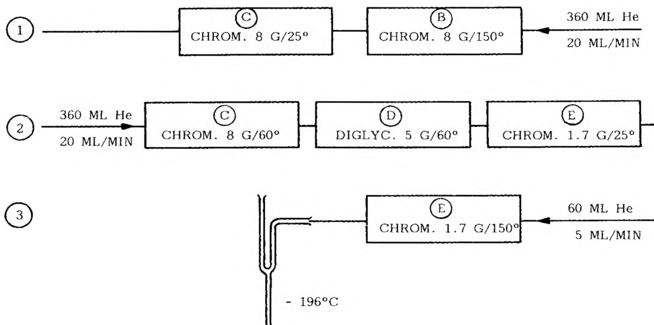
Fig. 7. Ethanol-free collection of headspace volatiles. Breakthrough volumes: ethanol, 380 ml/5 g of diglycerol (60°C); acetaldehyde, 920 ml/1.7 g of Chromosorb 102 (25°C). Desorption volumes: acetaldehyde, 320 ml/8 g of Chromosorb 102 (150°C); acetaldehyde, 60 ml/1.7 g of Chromosorb 102 (150°C).
