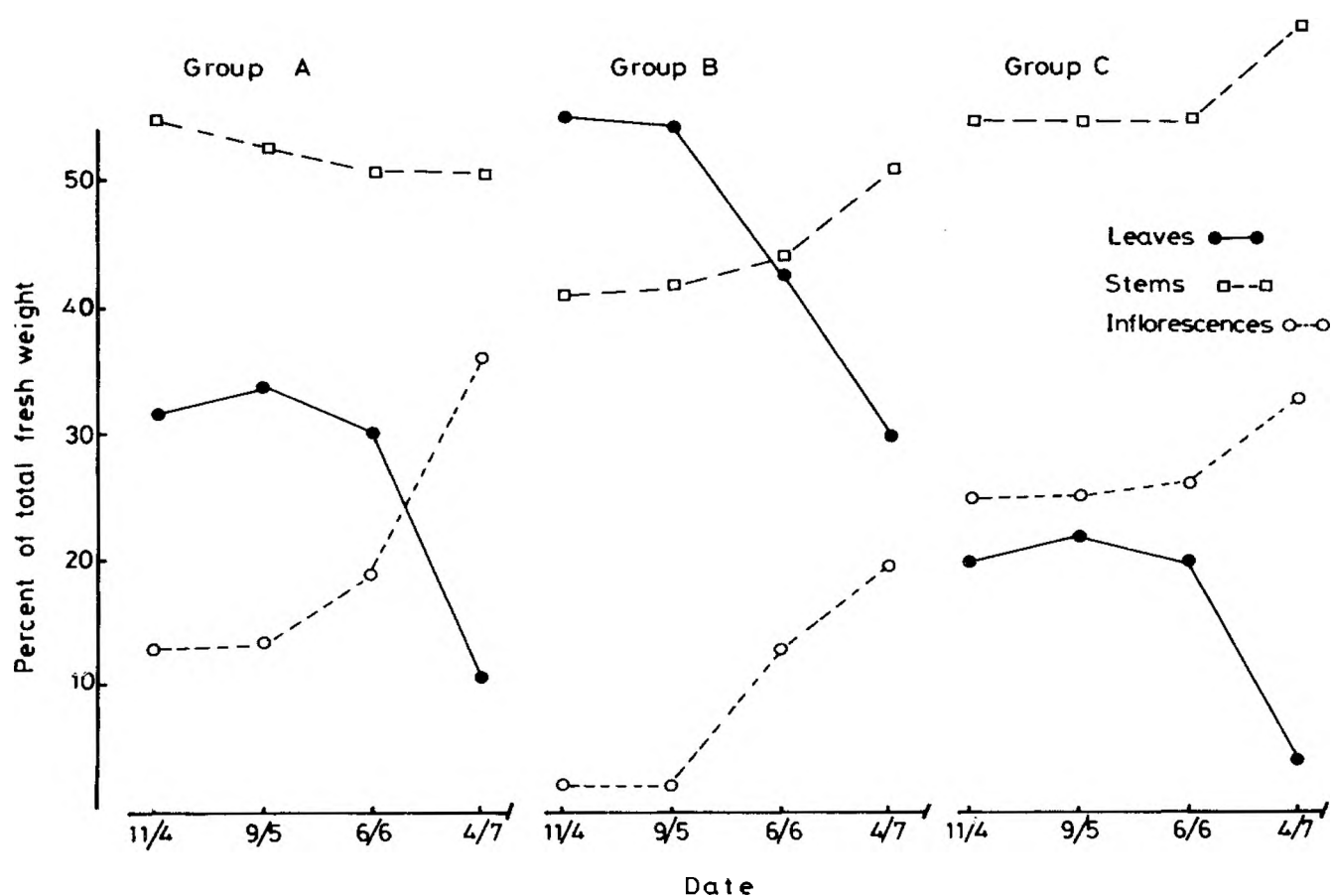
Fig. 2. Changes in various parts of the plant (percentage of total weight) during the growth of three Origanum vulgare groups.
