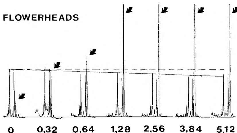
Fig. 13. The effect of the matrix on the amounts of the components in chamomile flowerheads after addition of various amounts of \alpha -bisabolol (arrow). Abscissa: added amount of \alpha -bisabolol \times 10^{-2} mg.
