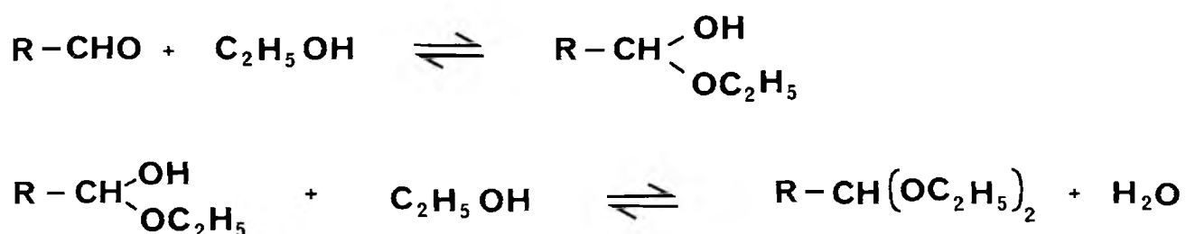
Fig. 1. Reactions in diethylacetal formation.
