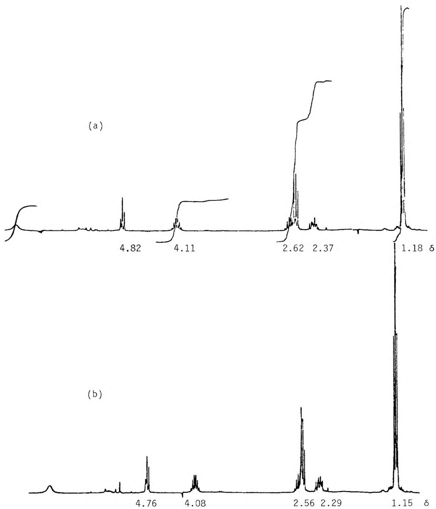
Fig. 2. NMR spectra of racemic 4-isopropylaminocarbonyl- \gamma -butyrolactone. (a) neat; (b) in presence of TFAE
