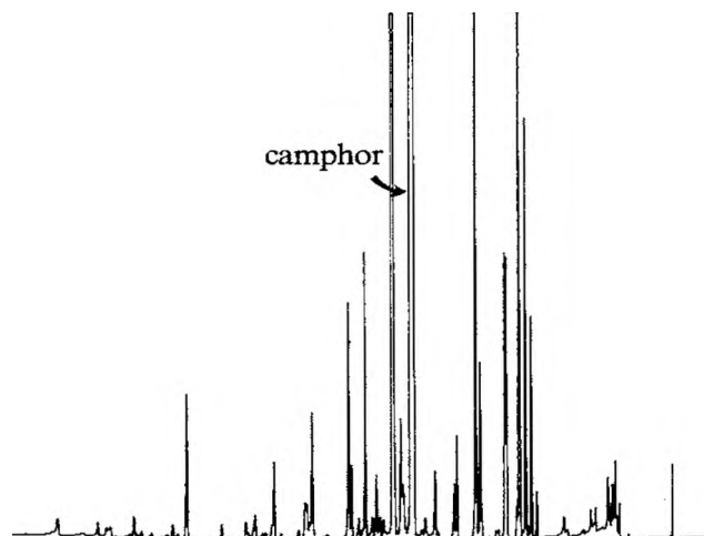
HSGC: Chemotypes of Tanacetum vulgare .
