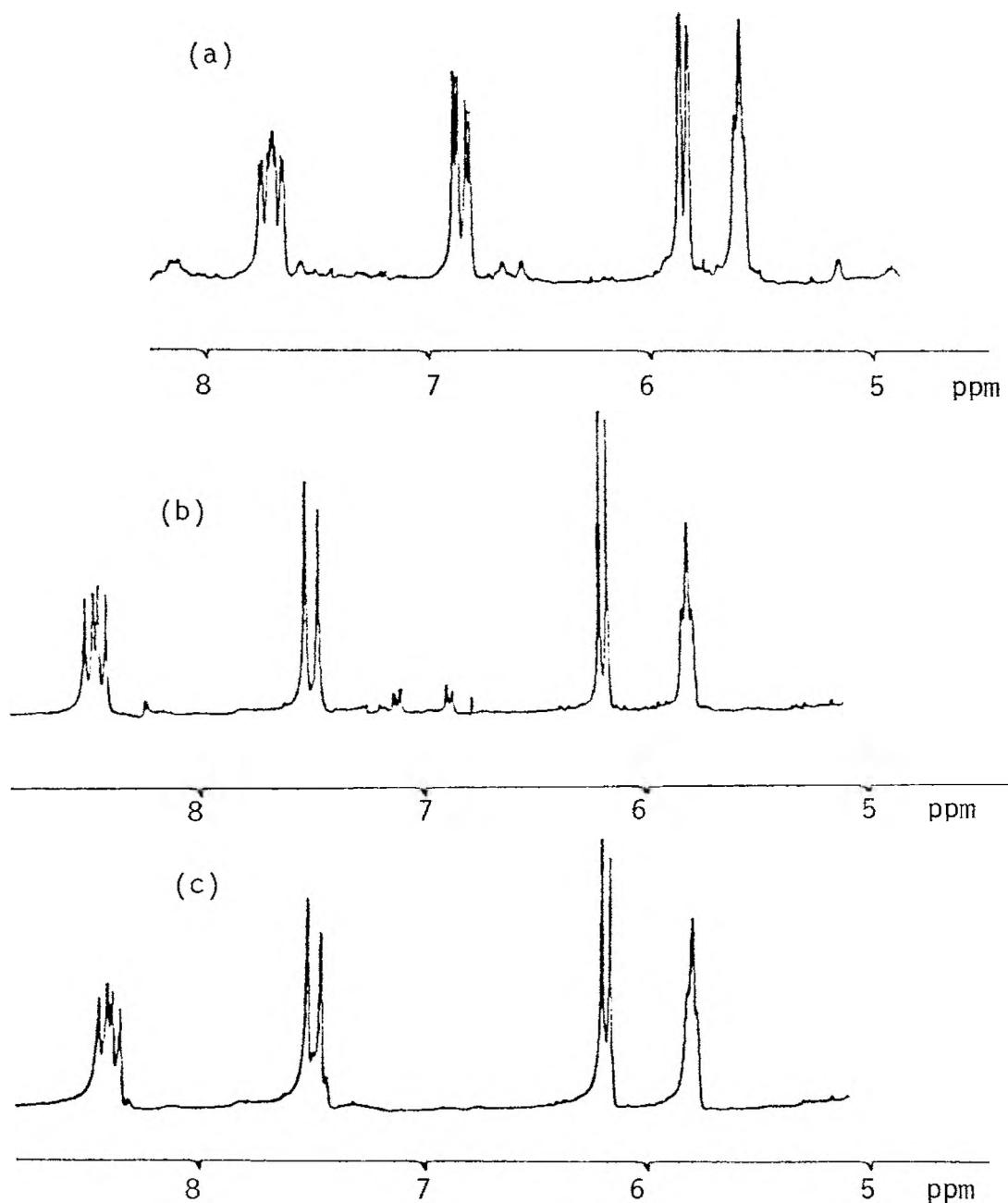
Fig. 1. NMR spectra of (a) synthetic racemic linalool, (b) natural linalool from sweet basil oil and (c) natural linalool from coriander oil, in presence of \text{Eu}(\text{hfbc})_3 .
