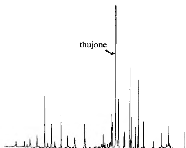
Fig. 7. Chromatograms obtained by HSGC showing four chemotypes of Tanacetum vulgare .
