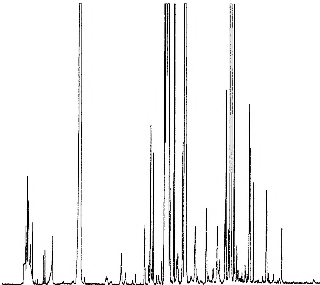
Fig. 3. Headspace analysis of tea aroma by cryofocusing. Perkin-Elmer Sigma 2000, HS-100; column, fused silica (50 m x 0.32 mm) coated with SE-54; temperature program, 60°C (6 min), then 60-140°C (6°C/min), after 4 min at 140°C, 140-200°C (20°C/min), then 200°C (25 min); carrier gas, Helium; sampling, splitless injection, 0.5 min; cryofocusing, -70°C, 200°C; sample, 400 mg tea (Earl Grey), 15 min at 80°C.
