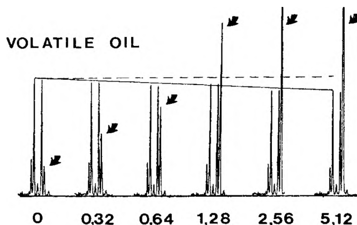
Fig. 12. The effect of the matrix on the amounts of the components in chamomile oil after addition of various amounts of \alpha -bisabolol (arrow). Abscissa: added amount of \alpha -bisabolol \times 10^{-2} mg.
