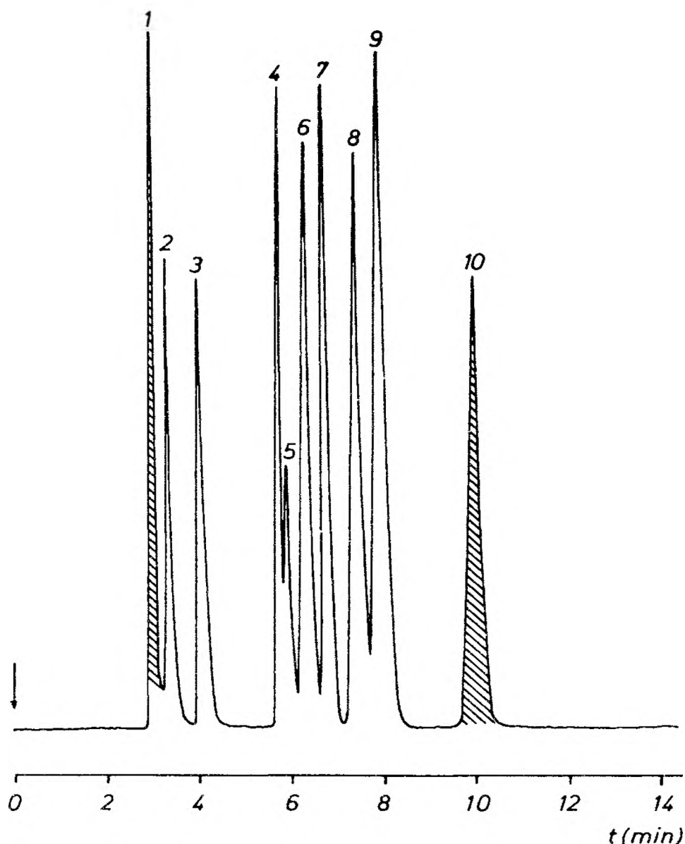
Fig. 10. HPLC separation of monoterpene hydrocarbons. Conditions: column, 30 cm x 4 mm i.d.; adsorbent, LiChroprep Si 60 (7 \mu m) with 4.8% water; eluent, n-pentane, 1.5 ml/min; temperature -15°C; UV detector. 1 = standard, 2 = \alpha -pinene, 3 = \beta -pinene, 4 = sabinene, 5 = limonene, 6 = \Delta^3 -carene, 7 = myrcene + cis- \beta -ocimene, 8 = trans- \beta -ocimene, 9 = p-cymene, 10 = standard.
