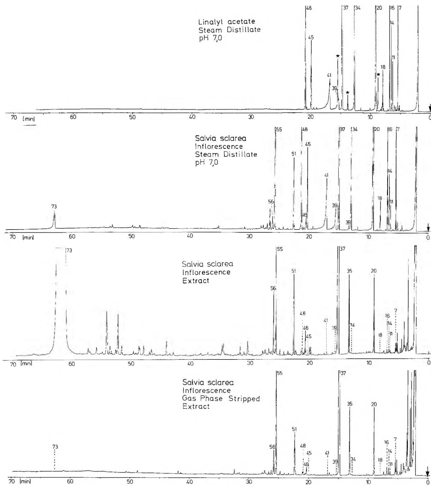
Fig. 4. Gas chromatograms of the hydrodistillate of linalyl acetate (pH 7.0) and of the essential oils of clary sage obtained by different methods. Column, capillary (30 m) coated with SE-30; oven temperature, 70-200°C (2.5°C/min); 7 = myrcene; 11 = limonene; 14 = cis - \beta -ocimene; 16 = trans - \beta -ocimene; 18 = terpinolene; 20 = linalool; 34 = \alpha -terpineol; 37 = linalyl acetate; 39 = nerol; 41 = geraniol; 45 = neryl acetate; 48 = geranyl acetate; 73 = sclareol.
