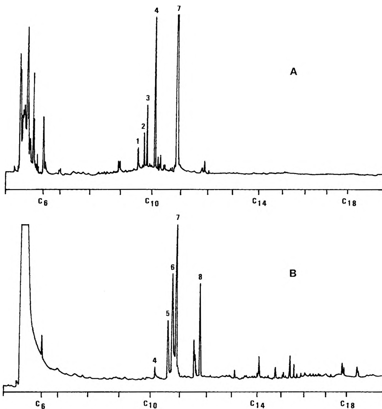
Fig. 5. Honeysuckle ( Lonicera periclymenum ): A. headspace; B. essential oil; 40 m OV-1 glass capillary column.
