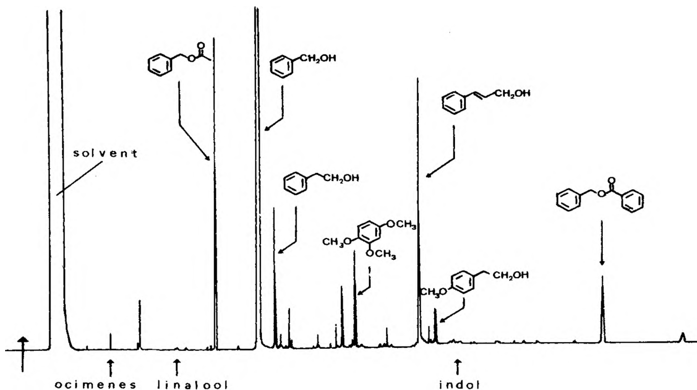
Fig. 1. Gas chromatogram of hyacinth absolute. Conditions: glass capillary column, 50 m x 0.3 mm, coated with UCON HB-5100; temperature program, 80°C (6 min) then 80-180°C (3°C/min); carrier gas, Helium, 3 ml/min; injection, 1 \mu l of a 0.5% solution in pentane on cold column.
