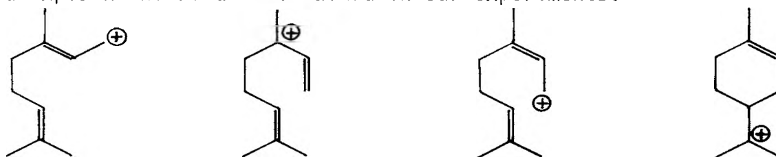
Fig. 2. Structural formulas of the intermediate cations (8). From the left to the right: geranyl, linalyl, neryl and \alpha -terpinyl cation.
