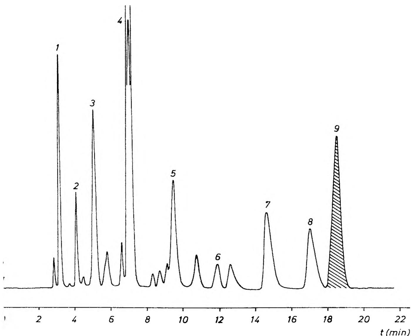
Fig. 11. HPLC separation of sesquiterpene hydrocarbons. Conditions see Fig. 10. 1 = \alpha -copaene, 2 = \delta -elemene, 3 = \beta -elemene, 4 = \beta -caryophyllene, 5 = \alpha -bergamotene, 6 = \beta -bisabolene, 7 = \alpha -humulene, 8 = \delta -cadinene, 9 = standard.
