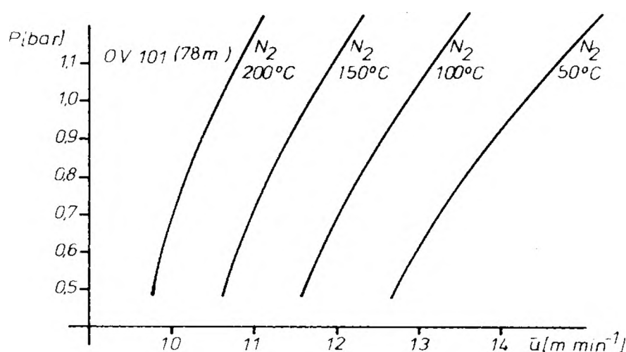
Fig. 7. Pressure and linear gas velocity at different temperatures.
