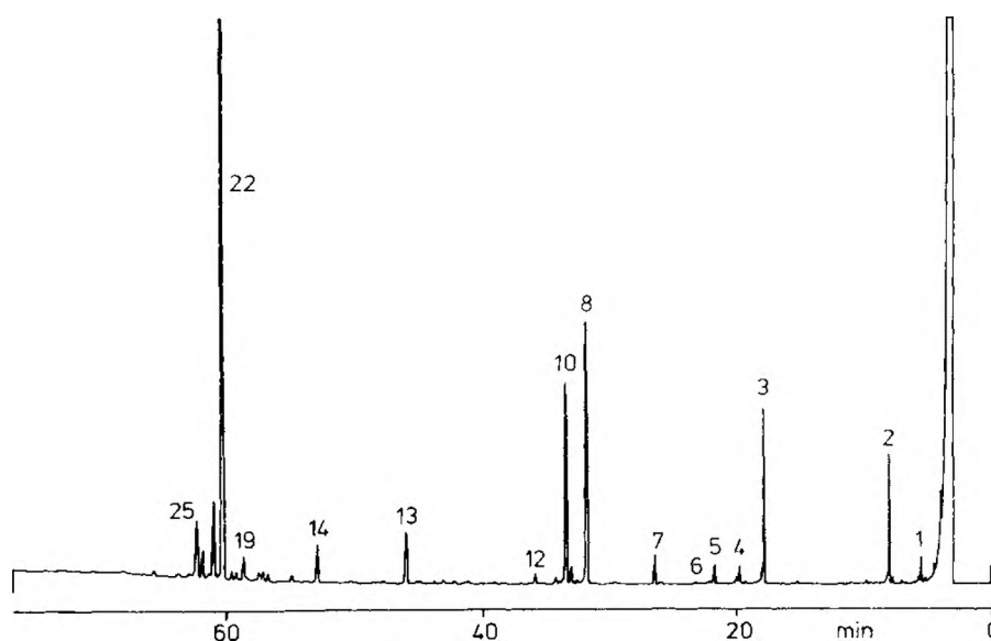
Fig. 2. Chromatogram of the volatiles in a 17 days old culture of C. populina . For gas chromatographic conditions, see under Material and Methods.
