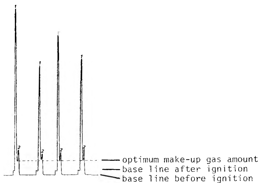
Fig. 6. FID response due to optimization with make-up gas.
