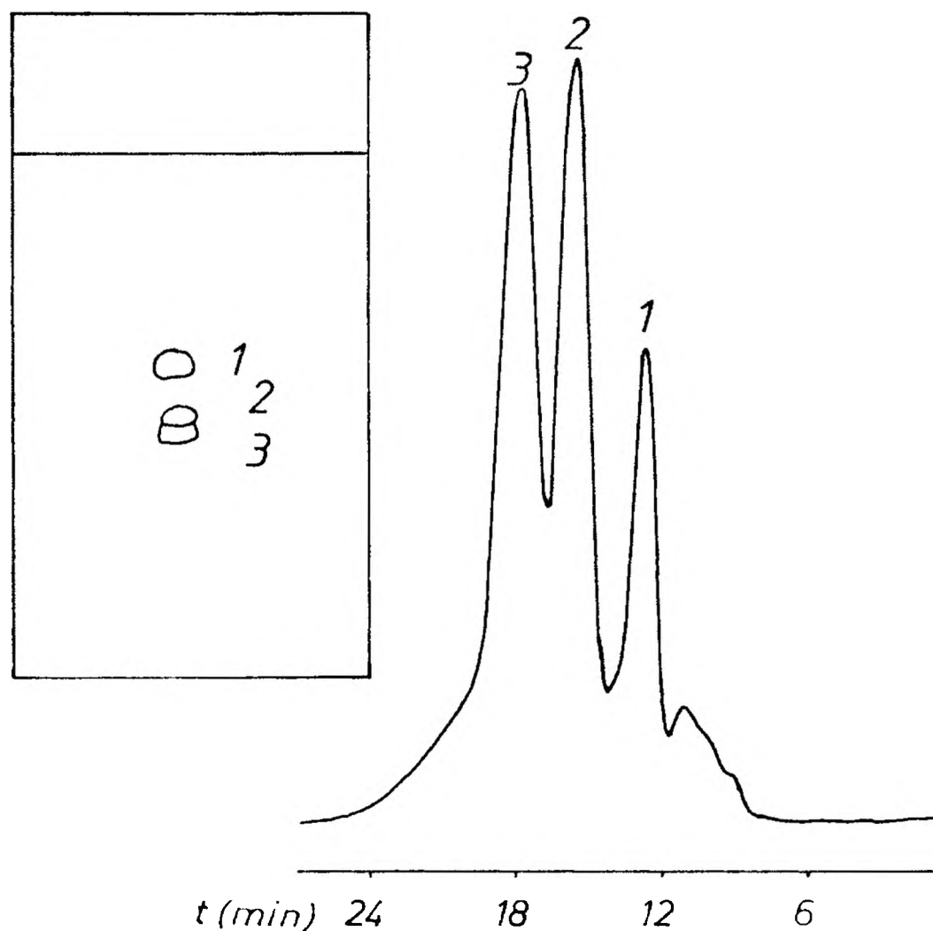
Fig. 6. TLC optimization of the mobile phase for preparative LC separation of Dictamnus albus fruit oil constituents. 1 = methyl cinnamate, 2 = neral, 3 = geranial.
