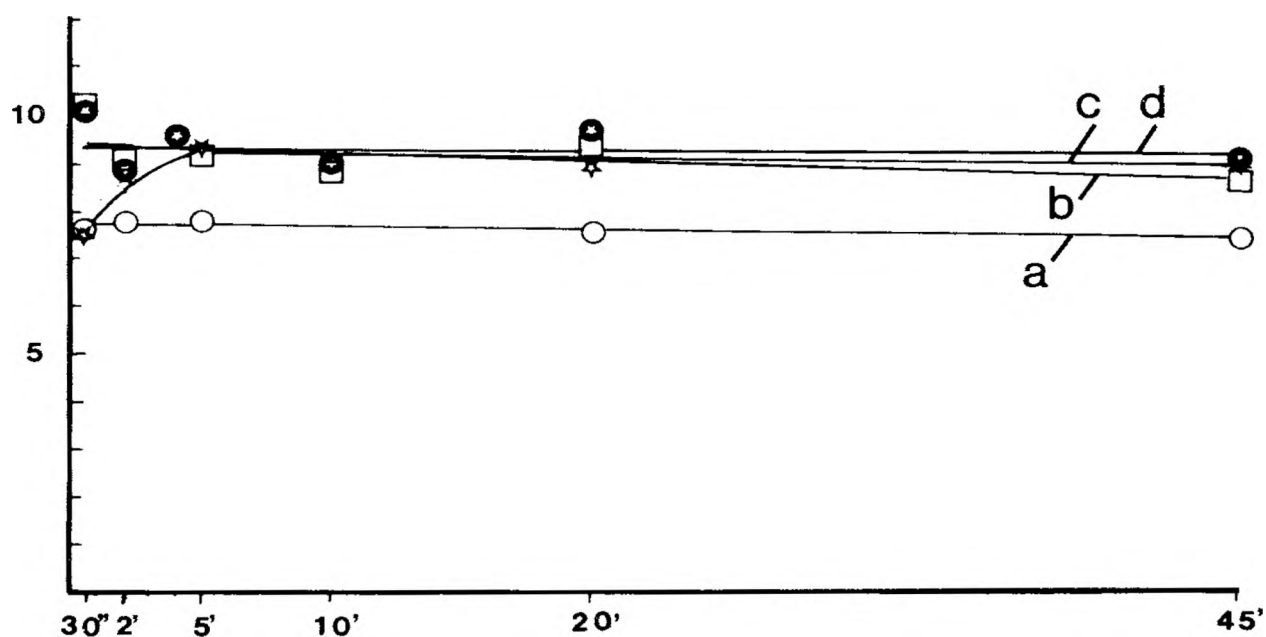
Fig. 2. The effect of equilibration period on the total peak area of the MTHC mixture in HSGC analyses at various temperatures: a = 60°C; b = 90°C; c = 120°C; d = 150°C. Abscissa: equilibration period; ordinate: peak area \times 10^4 .
