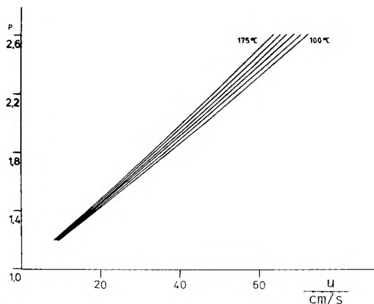
Fig. 8. Relation between adjusted pressure and average linear gas velocity at different temperatures.
