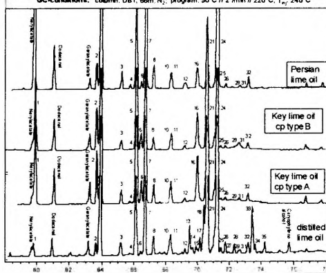
Fig. 2: GC-runs of different lime oils GC-conditions: column: DB1, 65m; N 2 ; program: 50°C // 2°/min // 220°C; T end : 240°C
