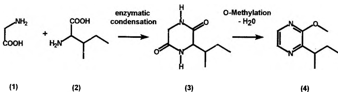
Fig. 1 Possible pathway of MMPP ( 4 )
