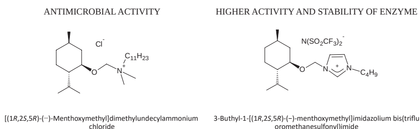
Fig. 1. Ionic liquids containing (–)-menthol derivative
