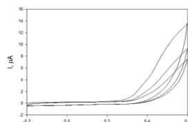
Figure 1. Cyclic voltammograms recorded on an essential oil-modified carbon paste electrode in phosphate buffer at pH 7.2. Potential scan rate 50mV/s.
