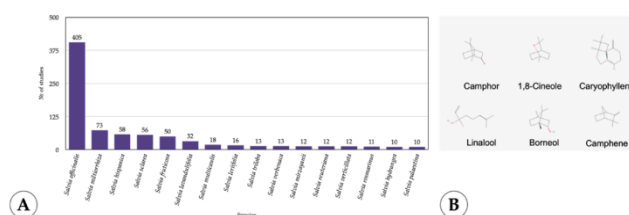
Figure 1: A – Numbers of essential oil studies for medicinally relevant Salvia species (only those with > 10 publications are shown). B – Most frequently reported major compounds for medicinally relevant Salvia species. Image source: : https://pubchem.ncbi.nlm.nih.gov/
